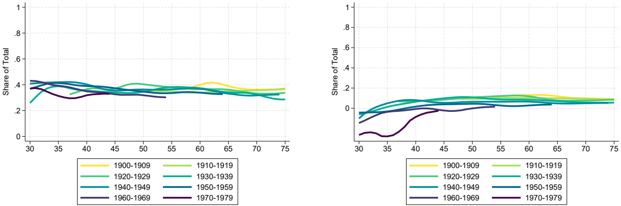
(a) Middle-40%
