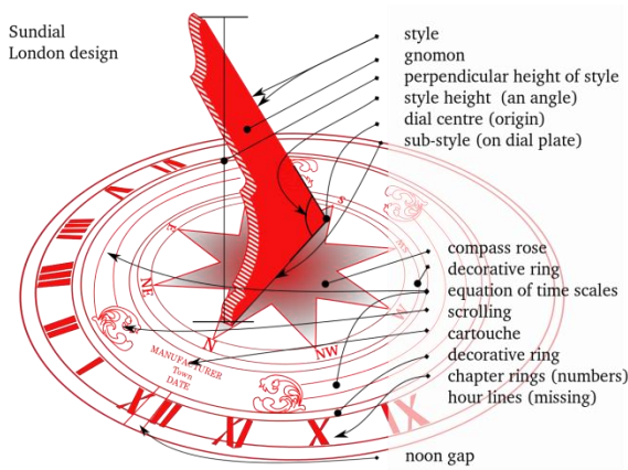
Figure 10 Cadran solaire
