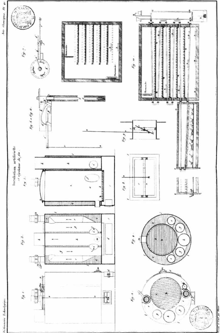
Figure 7. Bonnemain's hot water stove and chicken incubator ( Dictionnaire Technologique , vol. 11).
