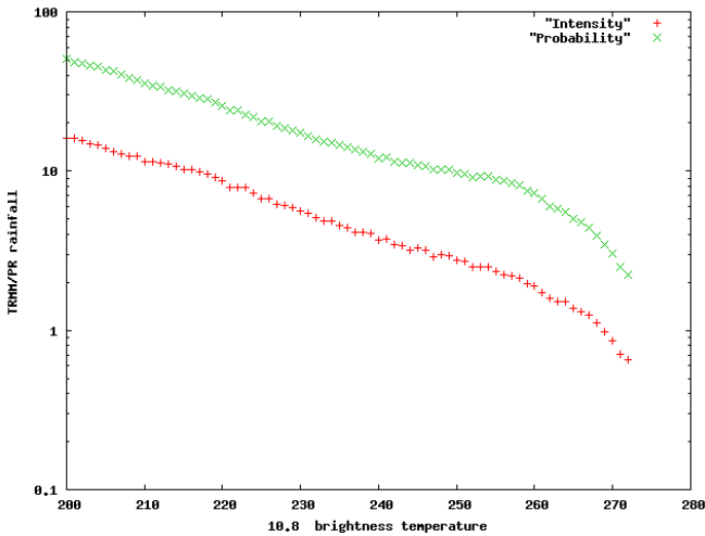
Fig. 1a. Empirical relationship between precipitation (rain rate and number of events) and 10.8 \mu\text{m} brightness temperature. The mean precipitation rate (red curve) is in mm/h and the mean number of rainfall events (green curve) is in percent. Both curves are plotted in logarithmic scale.
