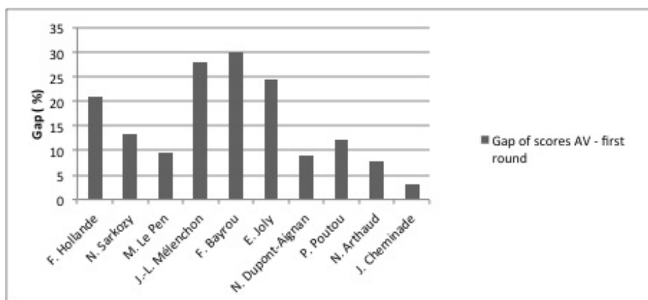
Figure 1 – Gaps of scores between AV and official results, France 2012
