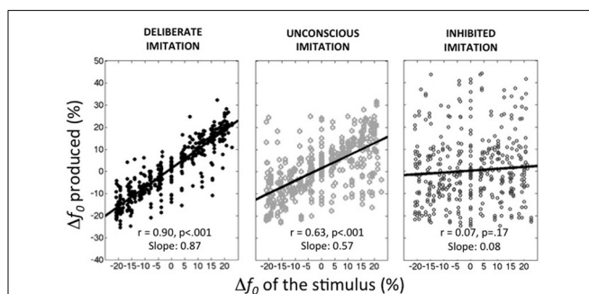
FIGURE 1 | Average behaviors observed in the three tasks of deliberate, unconscious, and inhibited imitation. Vowel stimuli were presented with 9 f_0 values, varying around the habitual average pitch of each participant. The y-axis represents how participants modified their produced f_0 from their habitual average f_0 (see Table 1 ).
