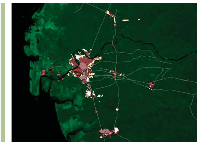
Figure 5. Urban growth of Surat (merger of two vector format spatio-temporal maps). Urban growth between 1990 (red) and 2001 (yellow) merged with a processed Landsat 7 ETM+ image.
