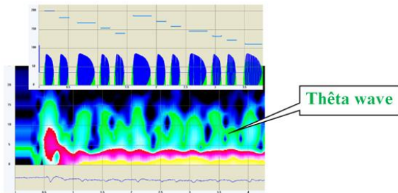
Fig. 3. Example of EEG spectral analysis (channel 28 or Pz) of evoked potential for a stimulus of a sequence of pure tones structured in groups of 3, the third tone being longer (top of the figure). Spectral analysis (bottom) shows Theta waves (in the range 4 Hz-10Hz) organized in a temporal structure corresponding to the stimulus structure [11].
