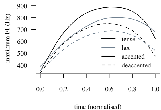
Figure 5: F1 trajectories (linear time-normalised) for the polysyllabic shortening experiment as a function of vowel density and accentuation
