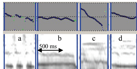
Figure 3: Examples of F0 contours and MFCC smoothed spectrograms for “unun”. F0 is in log scale from 110Hz ~ 440Hz (center dashed line at 220 Hz); spectrogram is in mel-scale 8kHz band. a) Fa_Fa_Fa ; b) FaFaFa ; c) FaFa? (pitch reset in the second “un” is unclear) ; d) Fa (F0 up-down motion is unclear)
