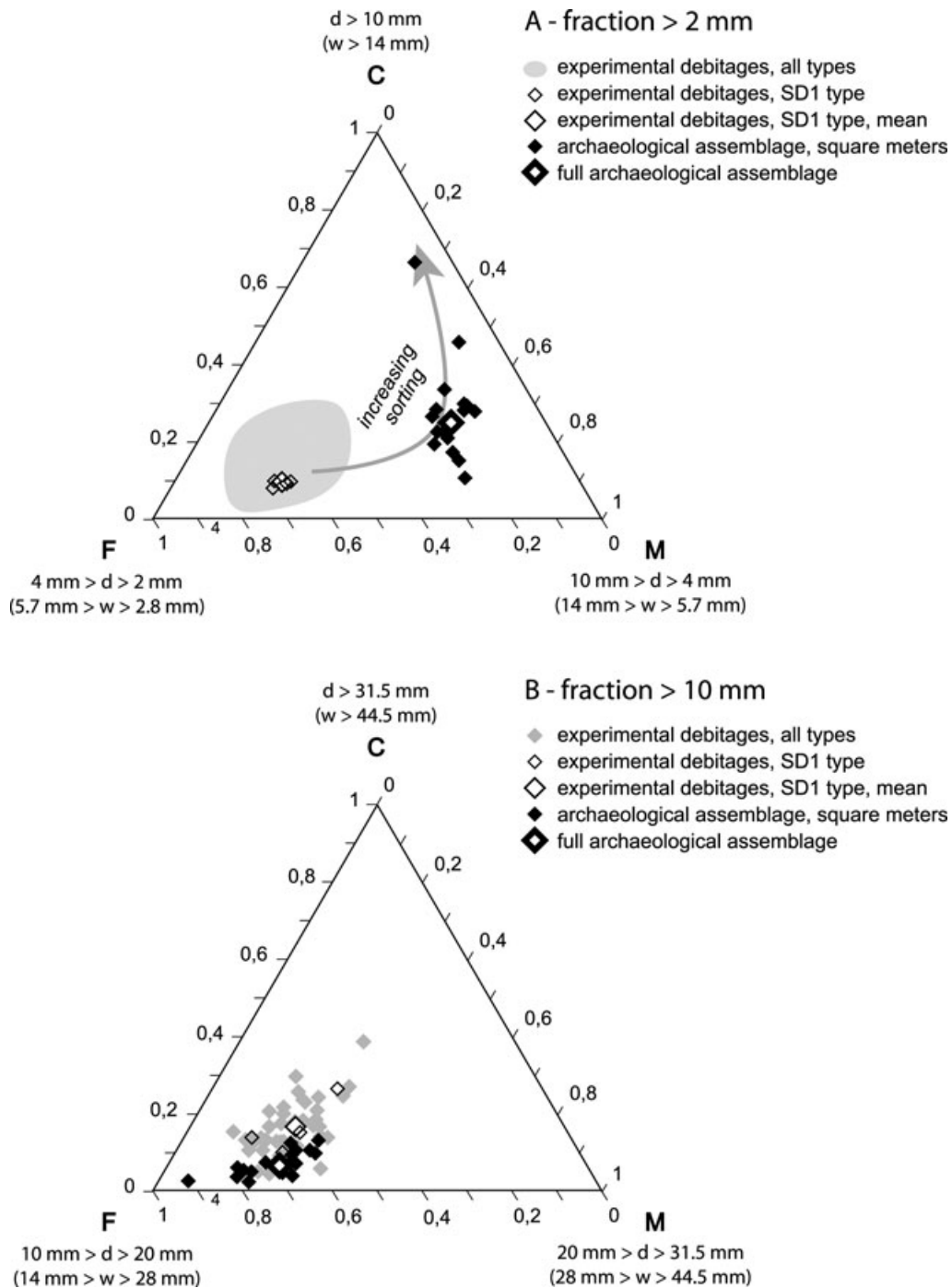
Figure 14 Particle size of the lithic material, triangular diagrams. (A) Fraction greater than d = 2 \text{ mm} ; the changing composition in relation to hydraulic sorting is indicated according to Lenoble (2005). (B) Fraction greater than d = 10 \text{ mm} .
