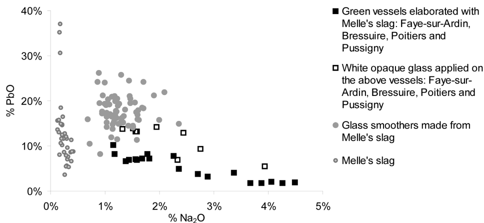
Fig. 9: Comparison of lead and sodium oxides contents of the beakers from Bressuire, Faye-sur-Ardin, Pussigny and Poitiers, and the lead-rich linen smoothers and slag from Melle. © CNRS, B. Gratuze.
