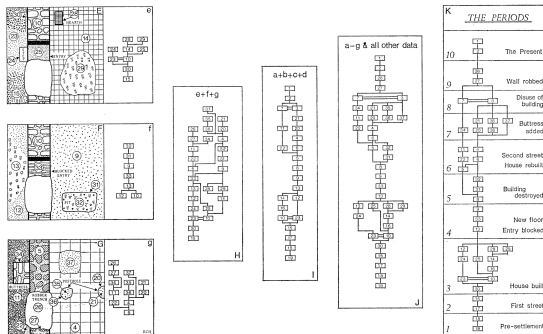
Figure 27 Plans E-G are reduced to the sequences e, f and g, which are combined in H. J presents the merger of I (see fig. 26), H, and all other stratigraphic information; the resulting stratigraphic sequence for this imaginary site is annotated in K.
