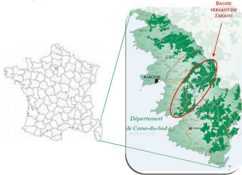
Figure 1: Geographical location of the Taravo river basin, French Corsica island
