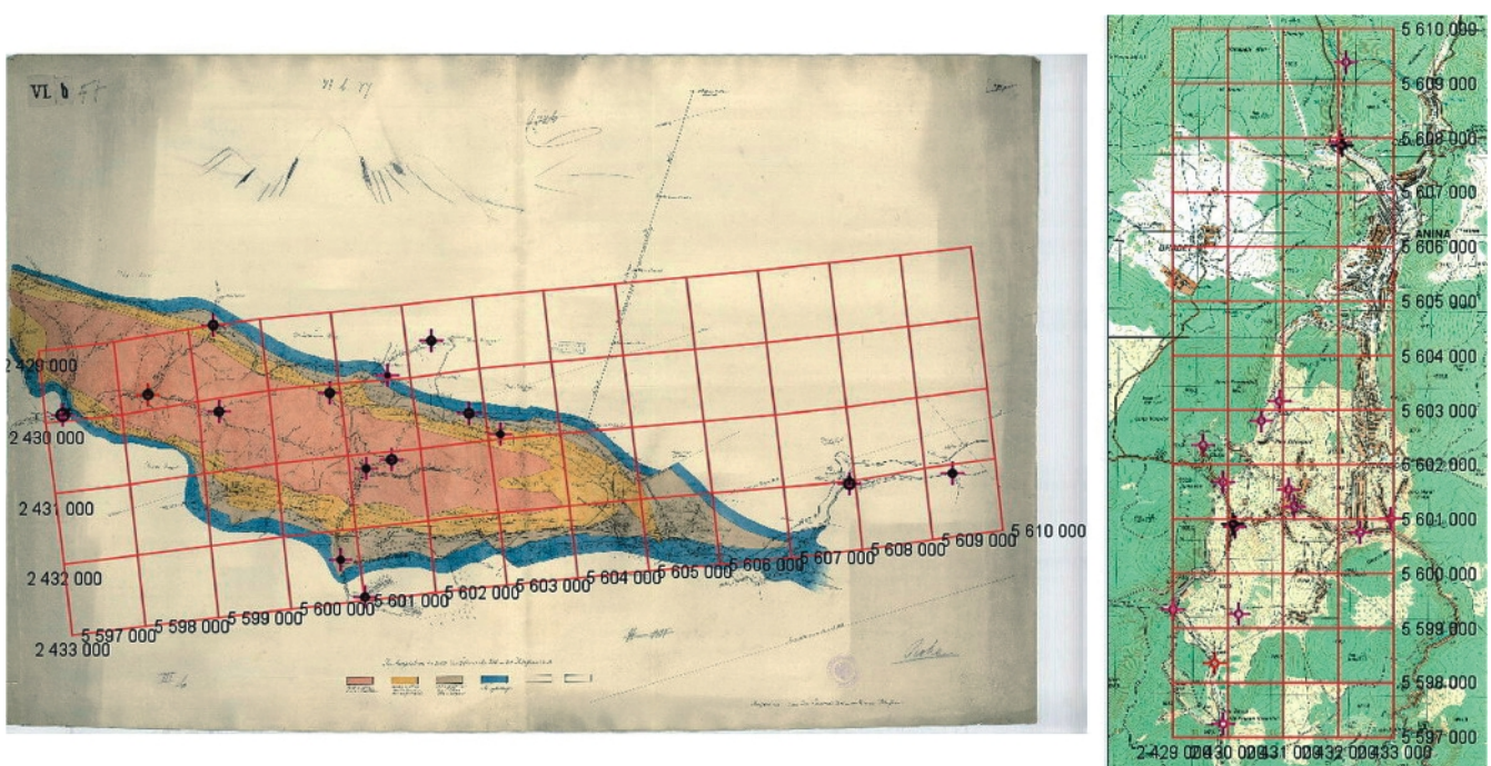
Figure 9: Analysis of the map by Roha (1867a[?]) visualised in MapAnalyst.
