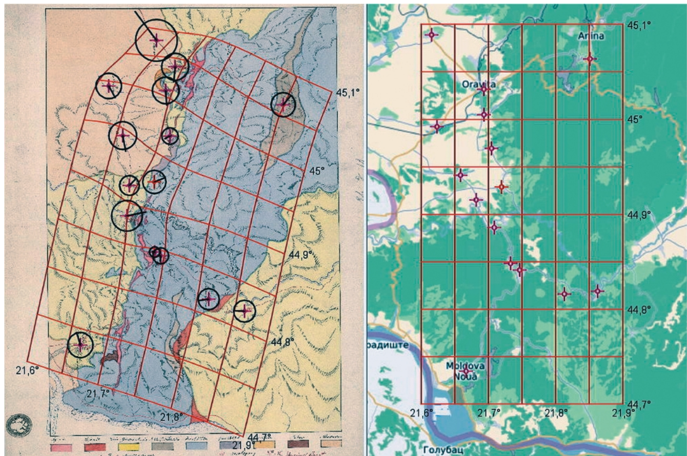
Figure 6: Analysis of the map Steierdorf Banat (***, ~1850) visualised in MapAnalyst.
