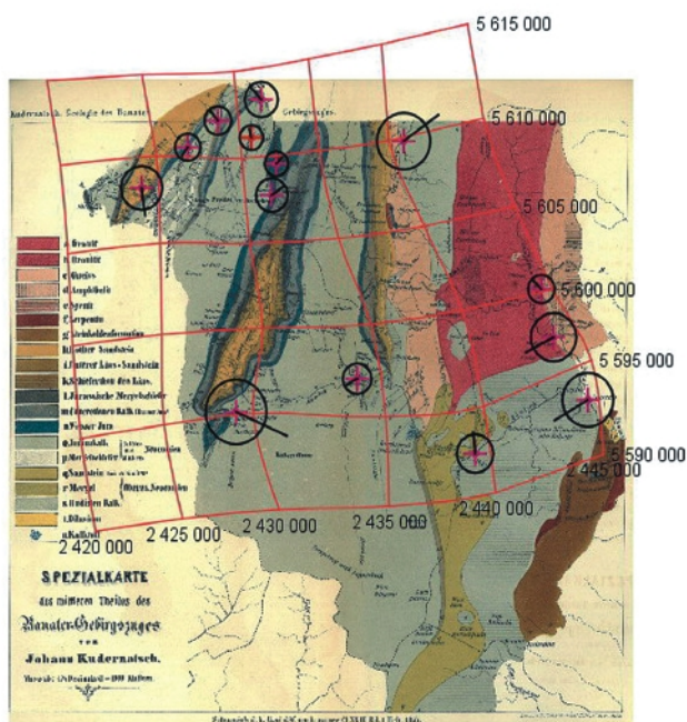
Figure 7: Analysis of the map by Kudernatsch (1857a) visualised in MapAnalyst.
