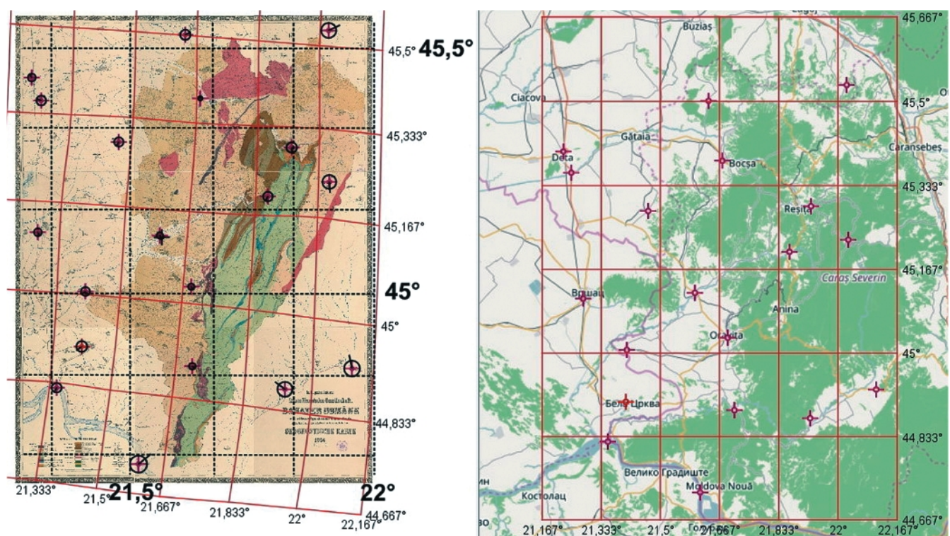
Figure 8: Analysis of the map Banater Domäne [...] (***) [Foetterle], 1860) visualised in MapAnalyst.
