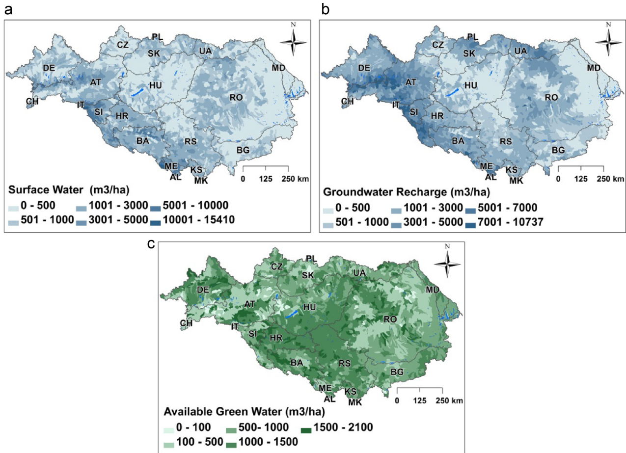
Fig. 4. Maps of renewable water in the Danube river basin estimated by the model SWAT: (a) surface water; (b) groundwater recharge; and (c) available green water. (For interpretation of the references to color in this figure legend, the reader is referred to the web version of this article.)
