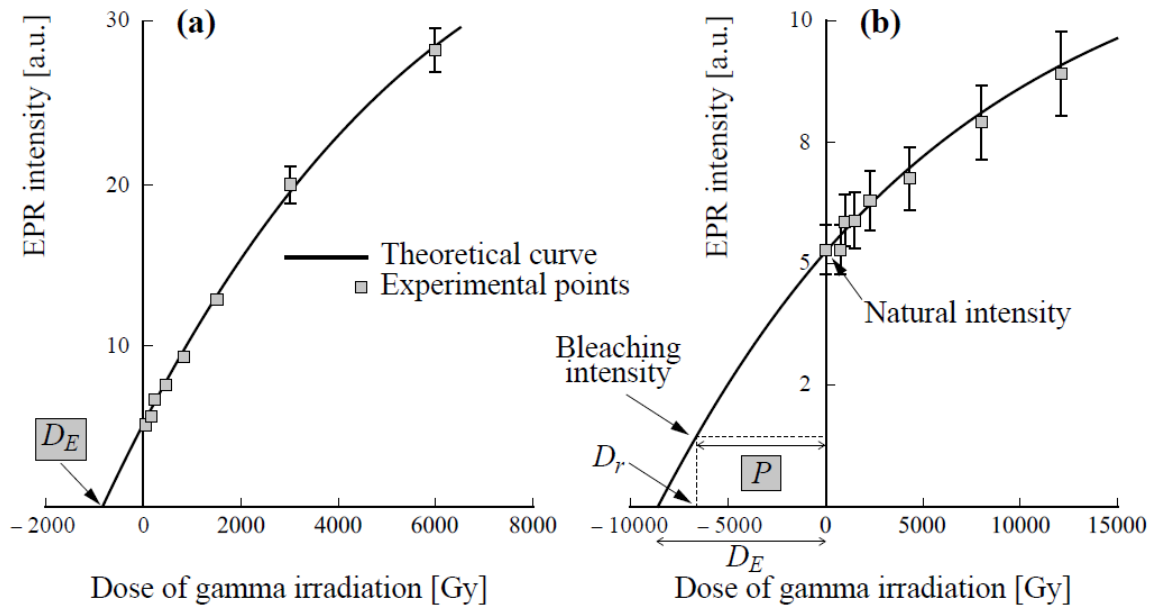
Figure 1.3. Sensitivity curves and calculation of the equivalent dose considered as the palaeodose. (a) fossilised dental enamel, (b) quartz. The dose due to bleaching must be subtracted from the total dose to obtain the archaeological dose. D_E = equivalent dose; D_r = residual dose; P = palaeodose (or archaeological dose) with D_E = D_r + P . The continuous line corresponds to calculations performed using equation [1.3].
