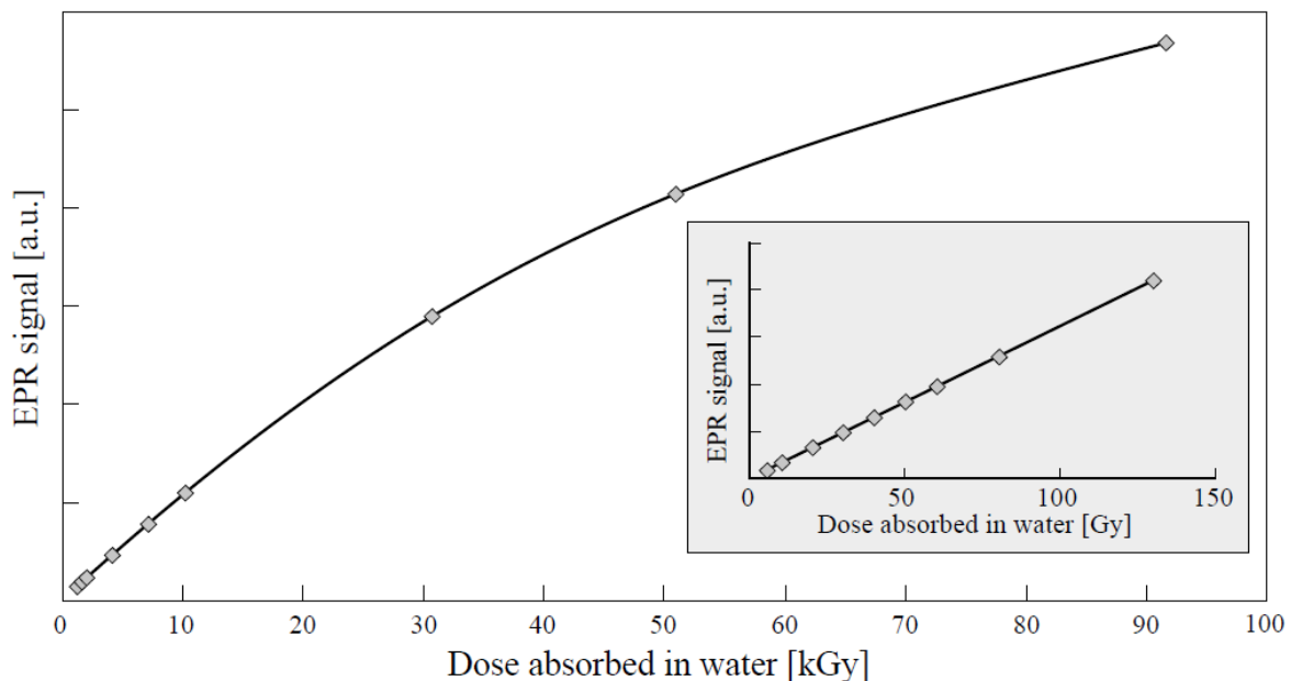
Figure 1.12 - Examples of alanine calibration curves for various dose ranges.
