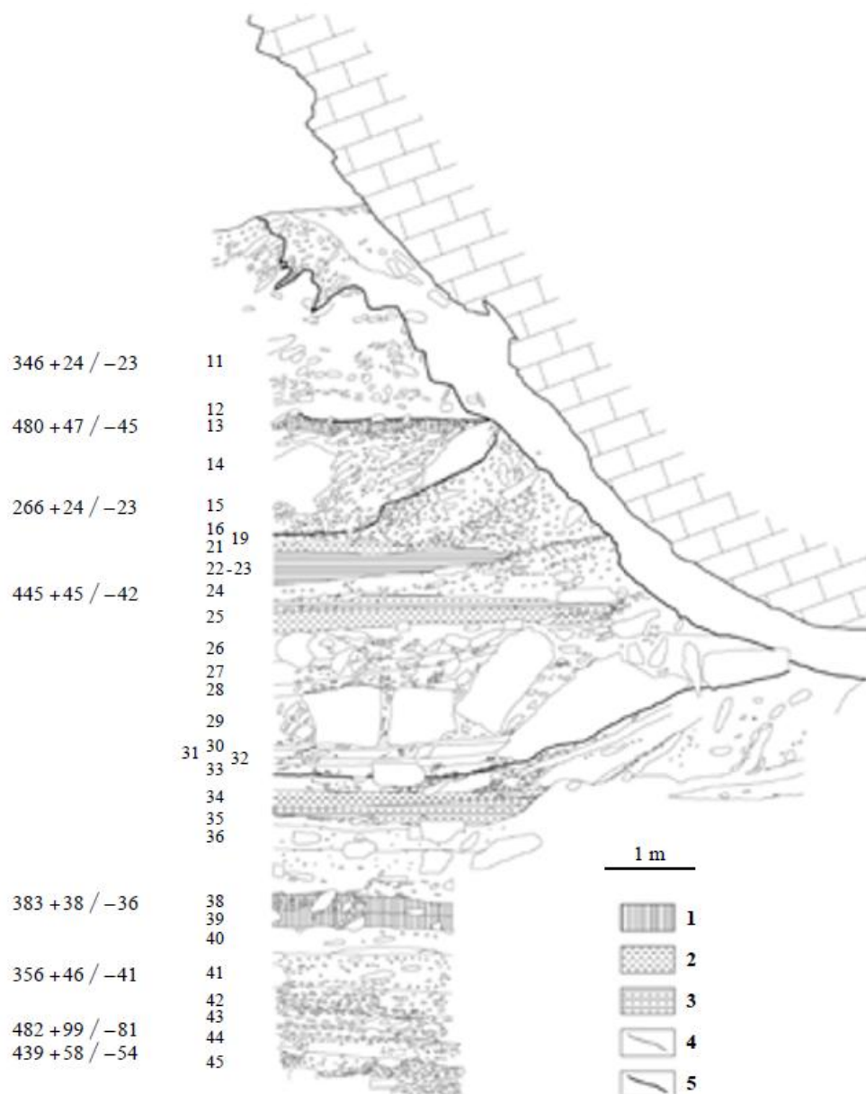
Figure 1.5. Longitudinal profile of the Visogliano site showing how the main geoarcheological levels, numbered from 11 to 45 are arranged. The ages determined by the EPR/U-Th method are expressed in ka on the left. 1: occupied soils, 2: löss levels, 3: altered löss levels, 4: limits of lithological units, 5: main discontinuities.
