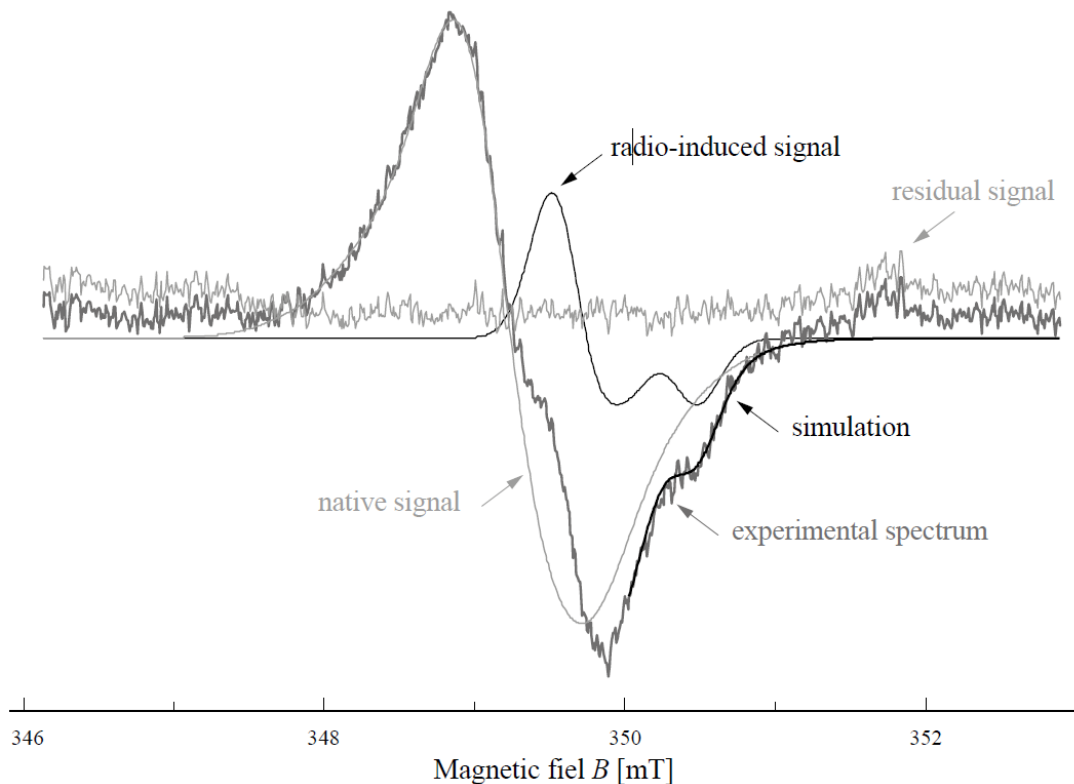
Figure 1.7. X-band spectrum for a sample of dental enamel irradiated at 500 mGy. Experimental conditions: room temperature, microwave power 2 mW. The simulation shows that it results from the superposition of a radio-induced component and a “native” component. The “residual signal” is the difference between the experimental spectrum and the simulation.
