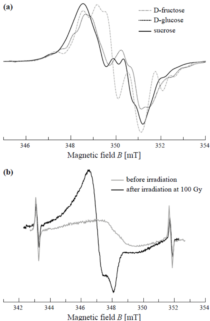
Figure 1.9. X-band EPR spectra for various irradiated samples. a) Samples of sucrose and the two monosaccharides composing it were irradiated at 100 Gy and their spectra were recorded. (b) Soda-lime glass, before and after irradiation at 100 Gy. Spectra were recorded at room temperature at 2 mW.
