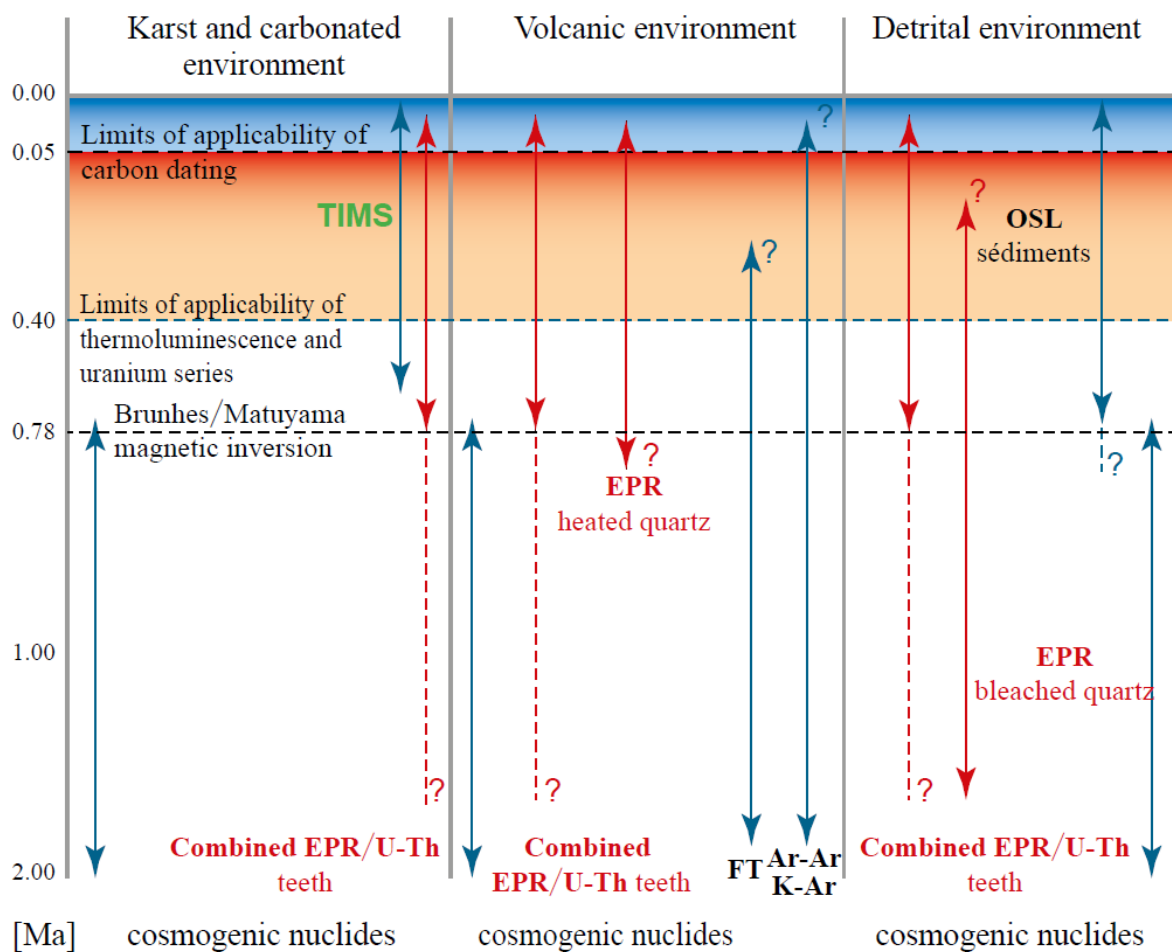
Figure 1.2. Comparison of the domains of application of the EPR method and the main methods used to date samples from the Quaternary period, depending on the different types of environment of the prehistoric sites. TIMS = U-Th method by thermo-ionisation mass spectrometry; FT = fission track method; Ar-Ar/K-Ar = argon-argon and potassium-argon methods; OSL = optically stimulated luminescence; U-Th = uranium-series method.
