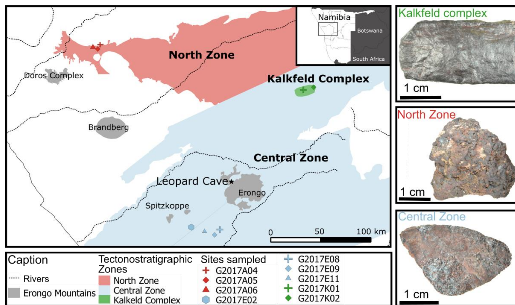
Figure 2. Geological context (left) and selected examples (right) of the Namibian geological samples analysed in the study. (double column, colour)
