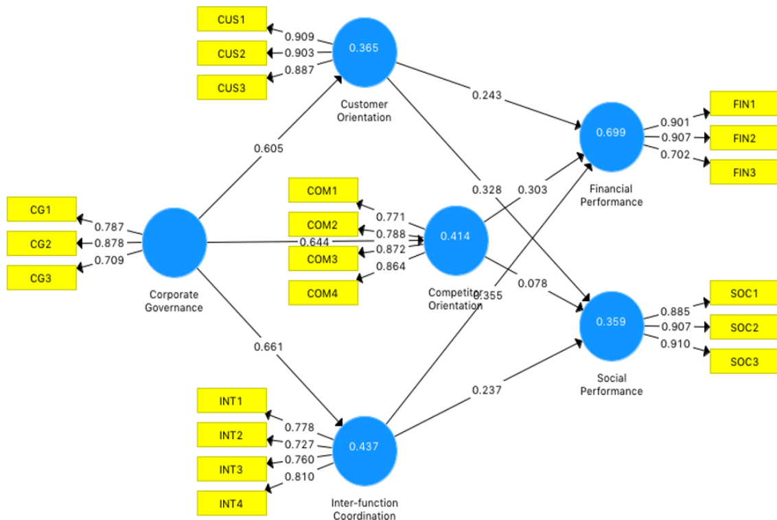
Figure 2. Path analysis
