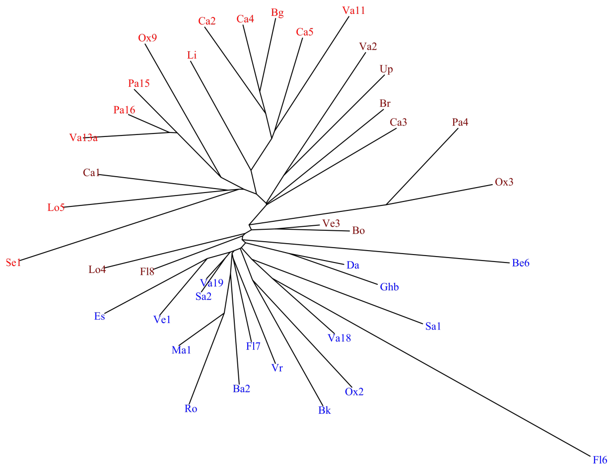
Figure 8: Centiloquium tree generated by the same method as fig. 6. The \alpha group is depicted in red (witnesses from the threefold version in lighter red), \beta in blue.
