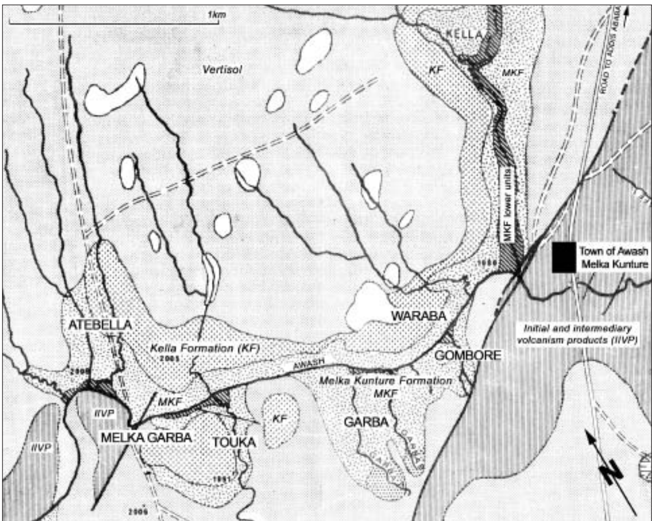
Fig. 2. Geological sketch map of the Melka Kunture area, after Täieb (1975) revised.
