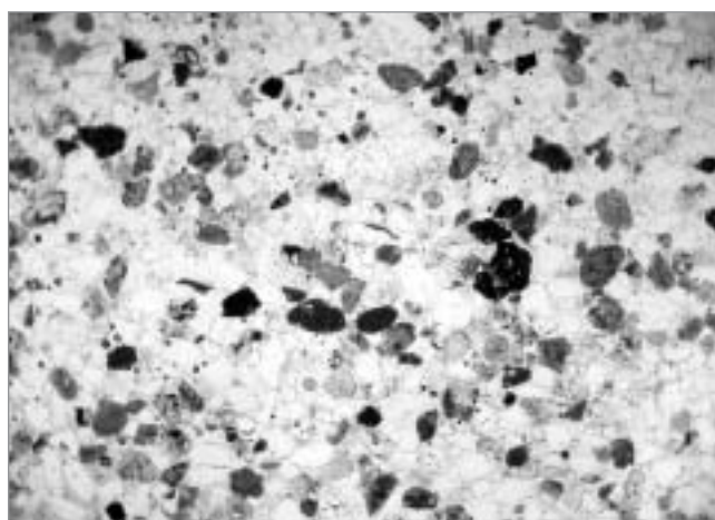
Fig. 29. Gombore II, sector 5, microscopic view of sample 2102 bottom, homometric sands, natural light.
