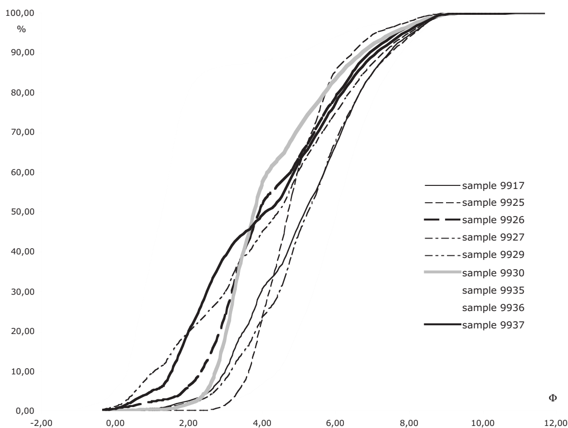
Fig. 13. Garba Gully, grain-size curves of the most representative layers.
