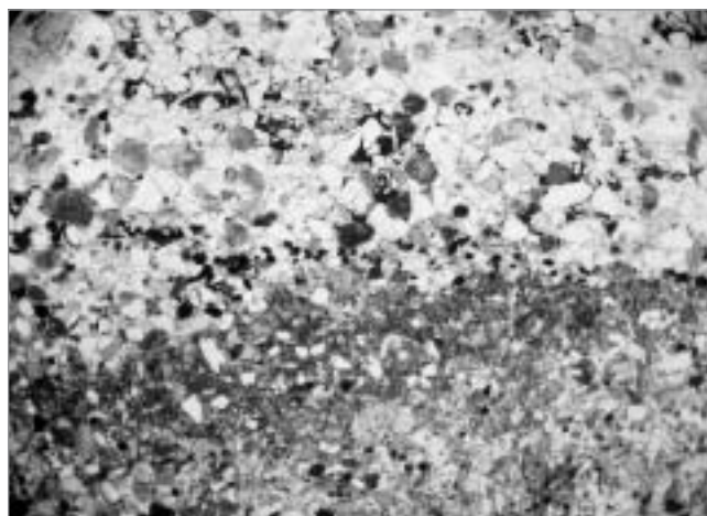
Fig. 28. Gombore II, sector 5, microscopic view of sample 2103 top, sands over silts, natural light.
