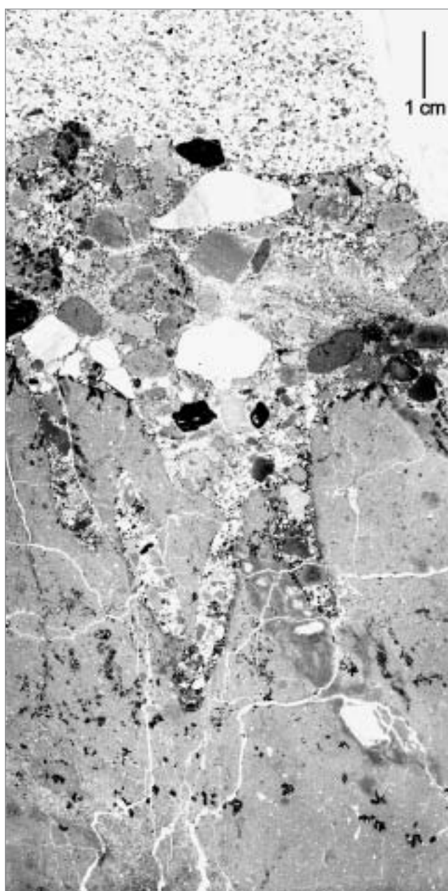
Fig. 18. Gombore I \gamma . Thin section from oriented sample 2149 in archaeological layer and enclosing beds, natural light. Cliché J.-P. Raynal
