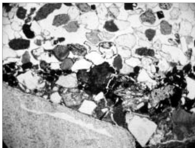
Fig. 20. Gombore I \gamma , microscopic view of sample 2149, the transition between the archaeological layer and the overlying sands, natural light. Cliché J.-P. Raynal
