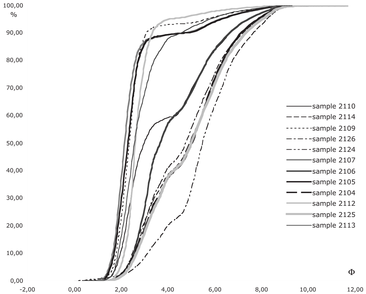
Fig. 32. Gombore II, sector 5. Grain-size curves of the most representative layers above the archaeological layer.
