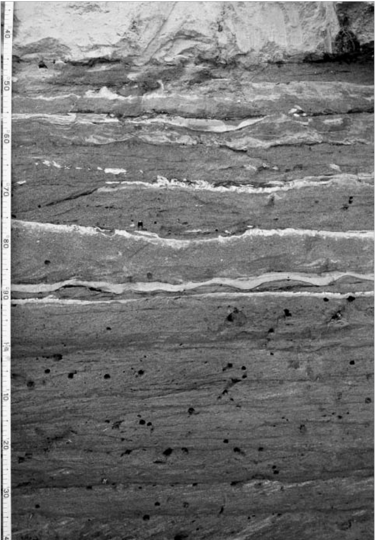
Fig. 22. Gombore Iy. Planar cross-bedded sands above archaeological layer, interbedded with fine redeposited tuffs.
