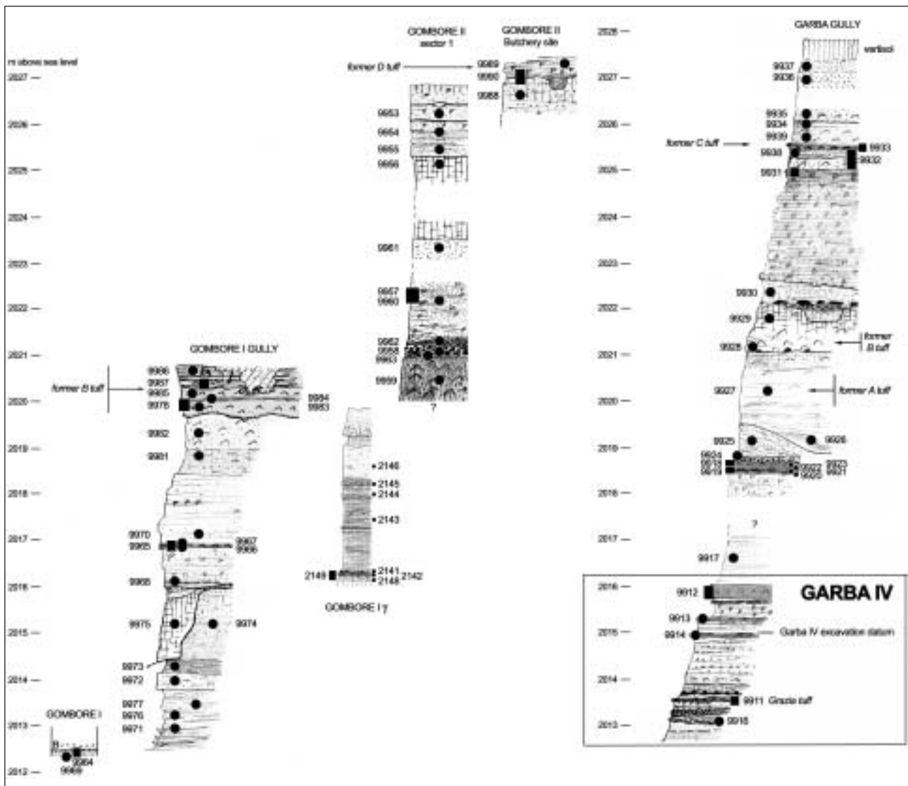
Fig. 3. Garba IV series in the context of the Melka Kunture Formation (logs in its lower part at Garba and Gombore).
