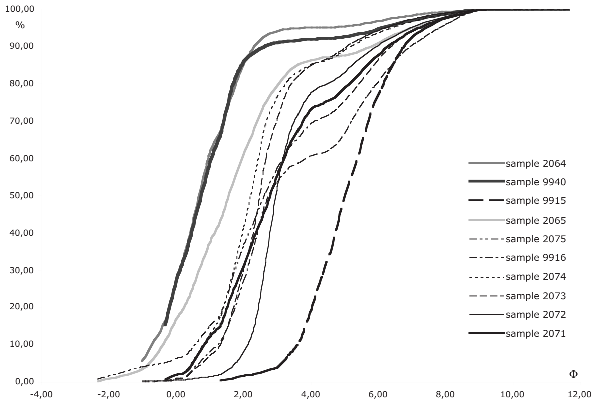
Fig. 6. Garba IV. Grain-size curves of lower beds up to archaeological Layer D.
