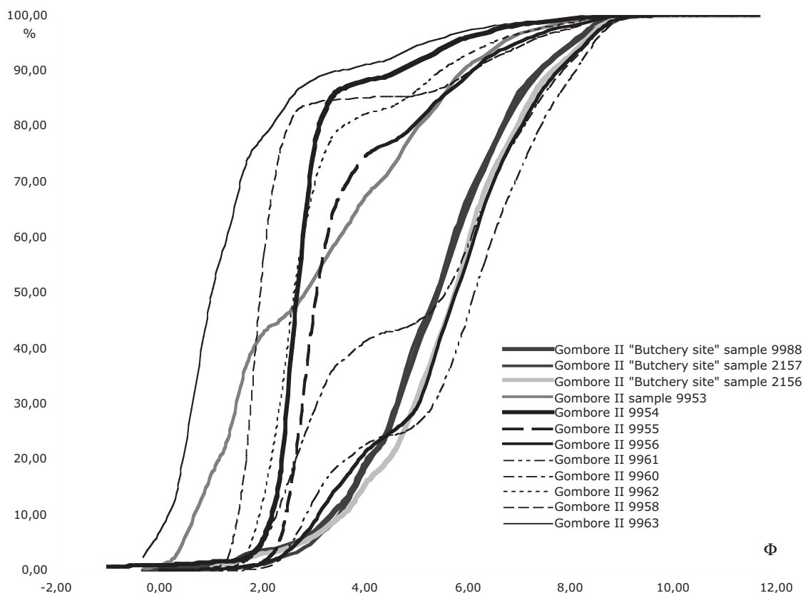
Fig. 33. Gombore II, sector 1. Grain-size curves of the most representative layers above the archaeological layer.
