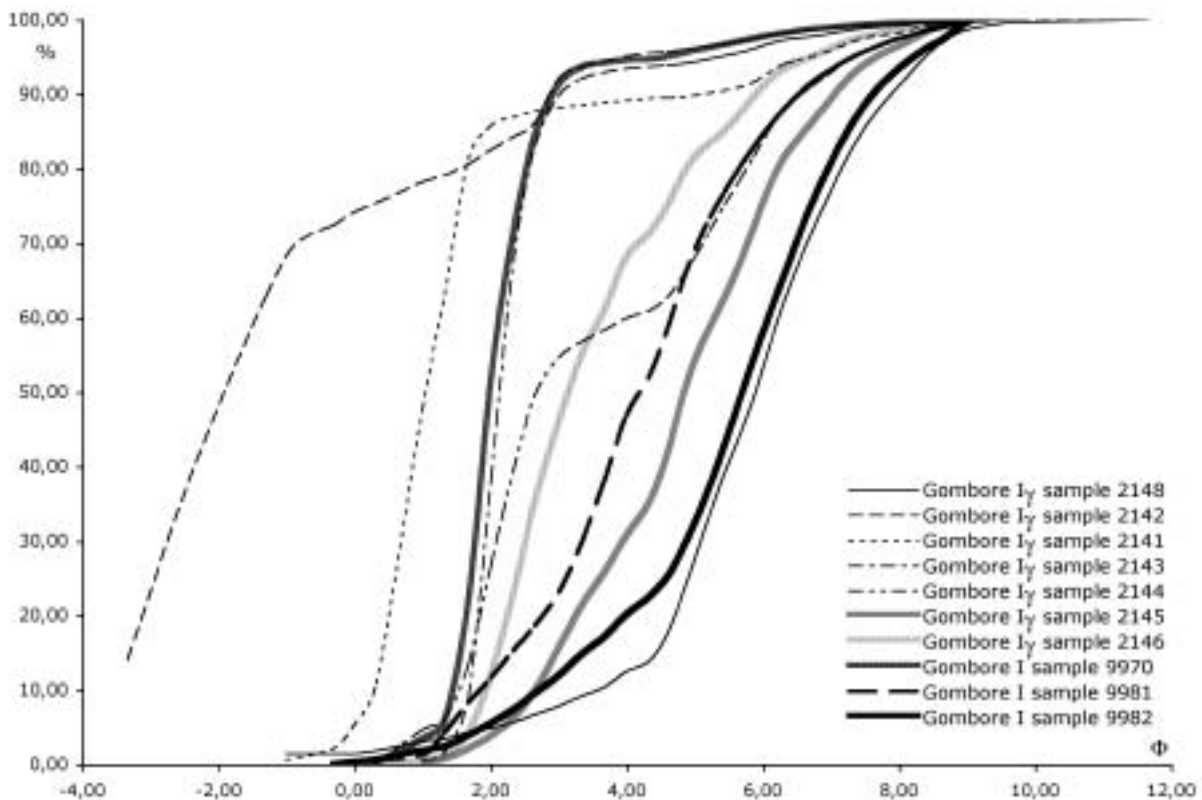
Fig. 16. Gombore I \gamma , grain-size curves of the most representative layers.
