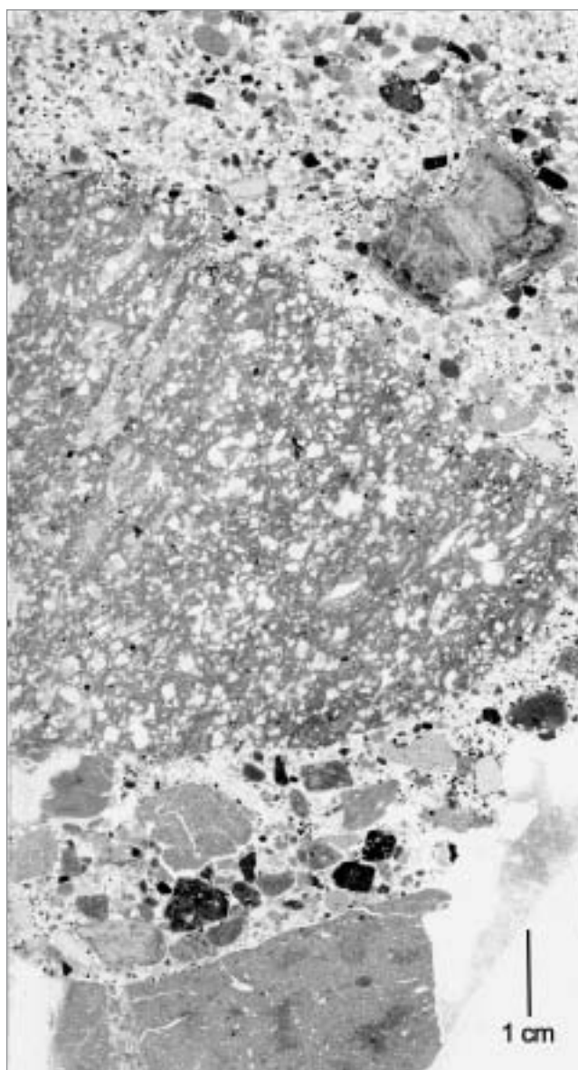
Fig. 7. Garba IV, sample 2054, thin section in beds 3.1 and 3.2, microscopic view in natural light.
