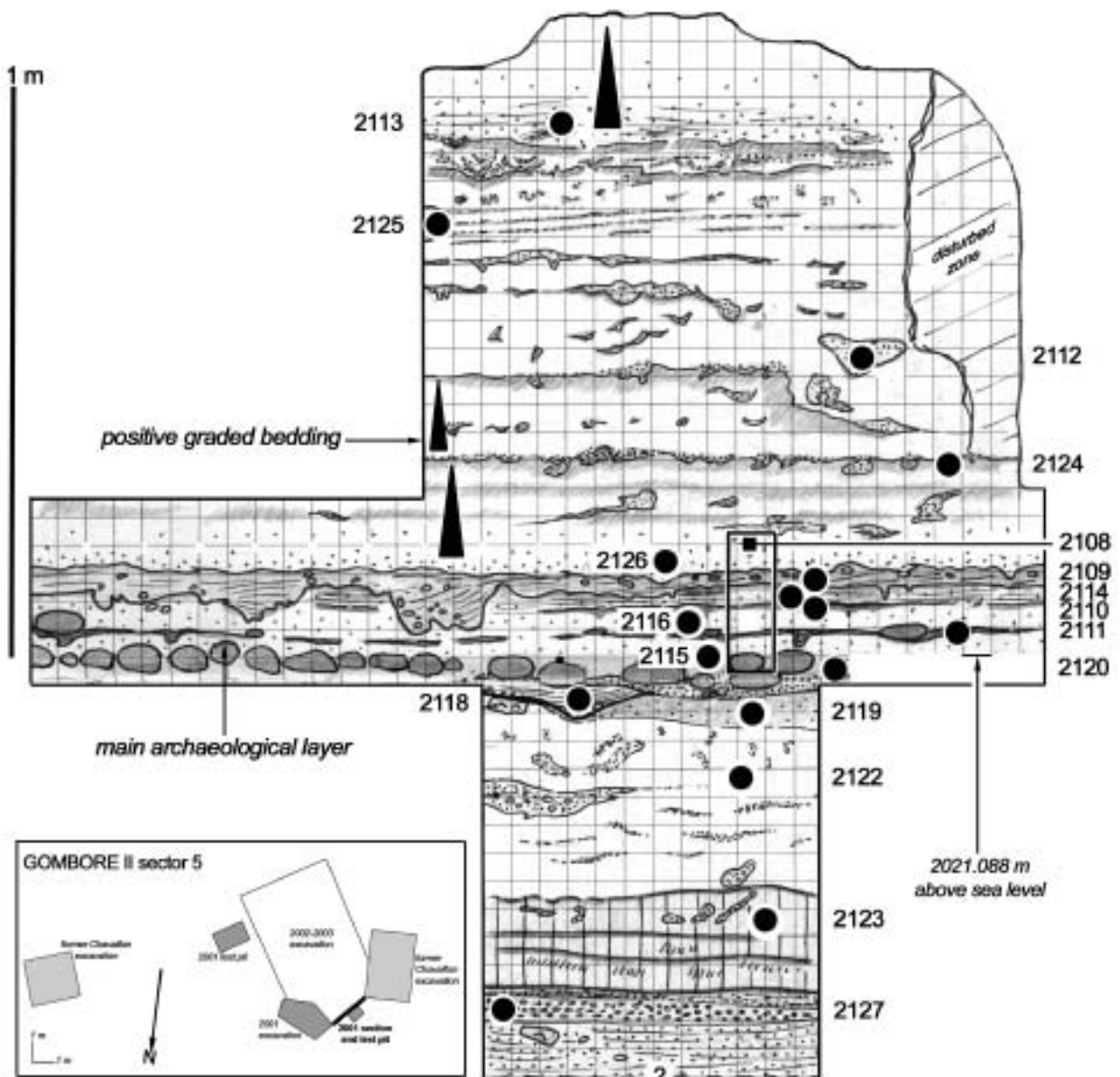
Fig. 23. Gombore II, sector 5. Section with sampling locations: black dots are sediment samples in bulk; black rectangle is oriented blocks sample for examination under the microscope.
