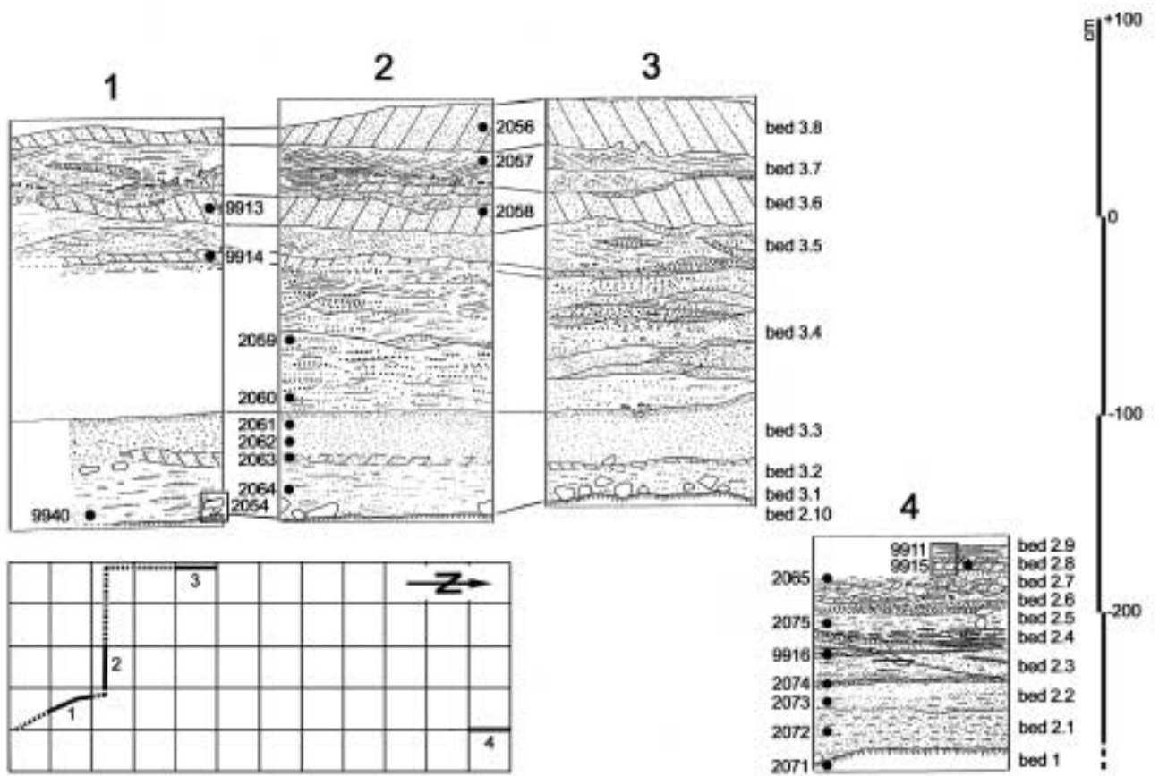
Fig. 5. Garba IV, stratigraphy and sampling locations.
