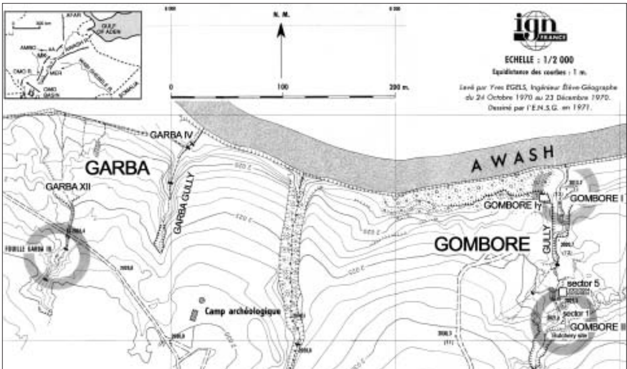
Fig. 1. Location map for the Melka Kunture area and detailed map of the Garba-Gombore sector (after Egels 1971).
