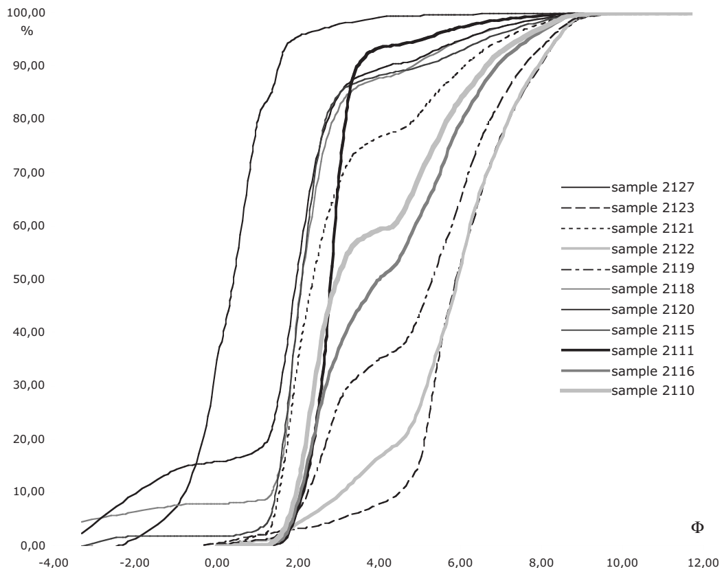
Fig. 24. Gombore II, sector 5. Grain-size curves of the most representative layers up to the archaeological layer and immediately above.
