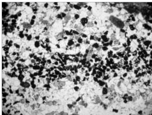
Fig. 25. Gombore II, sector 5, microscopic view of sample 2108 bottom, microbed of opaque minerals.
