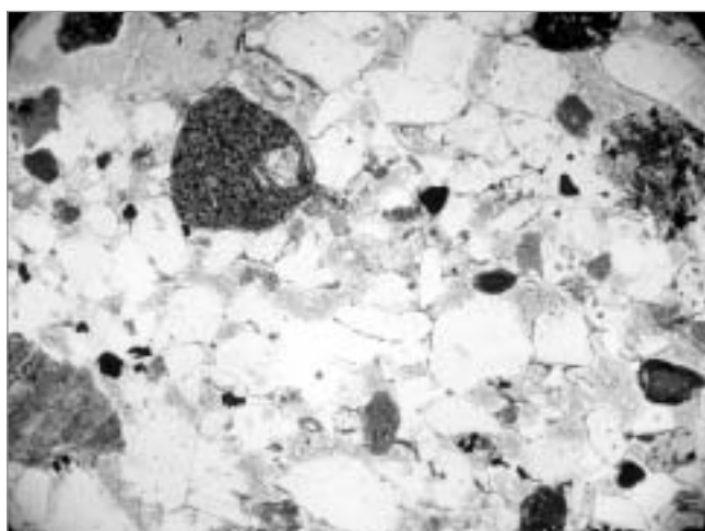
Fig. 9. Garba IV, sample 2054, thin section in bed 3.1, coarse sands, microscopic view in natural light.
