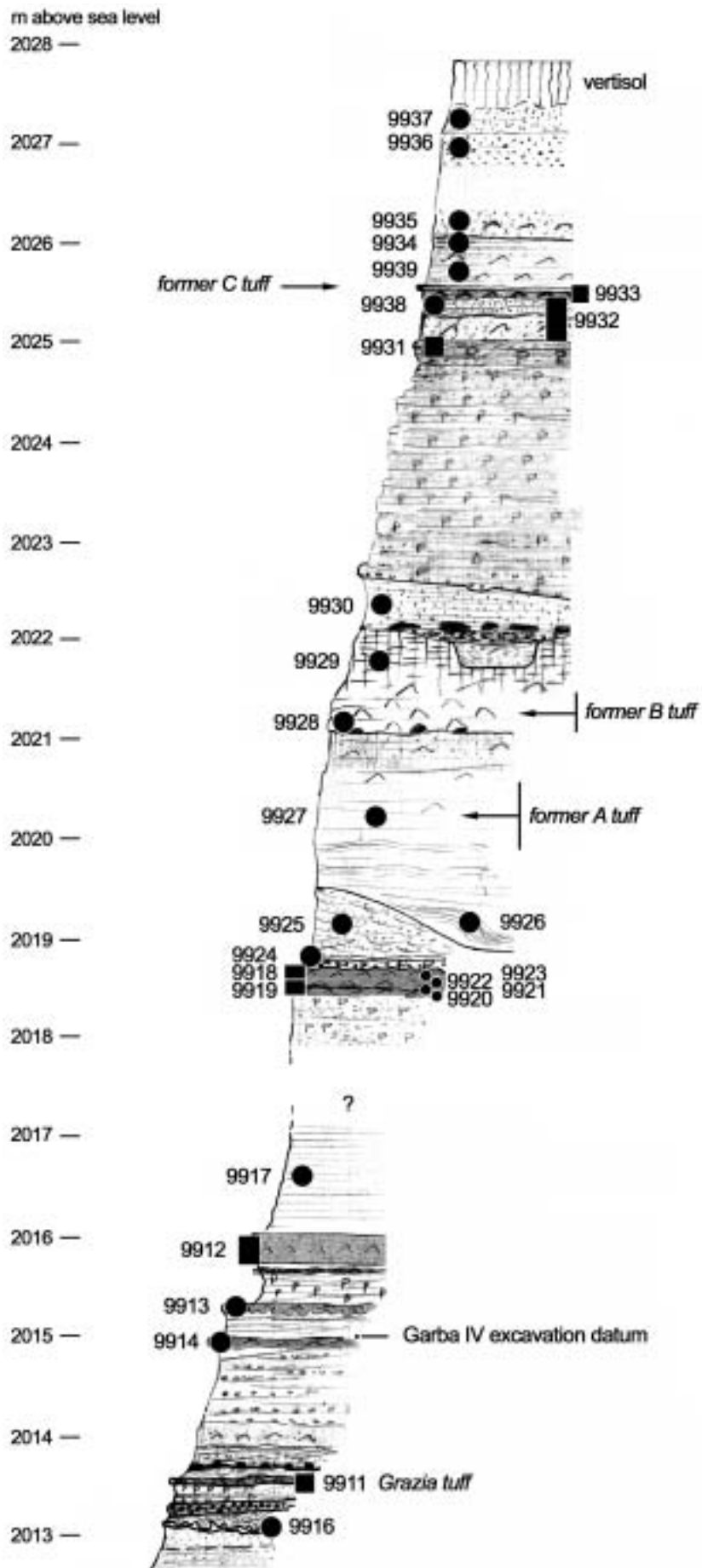
Fig. 12. The Garba IV and Garba Gully series: black dots are sediment samples in bulk; black rectangles are oriented blocks samples for examination under the microscope.
