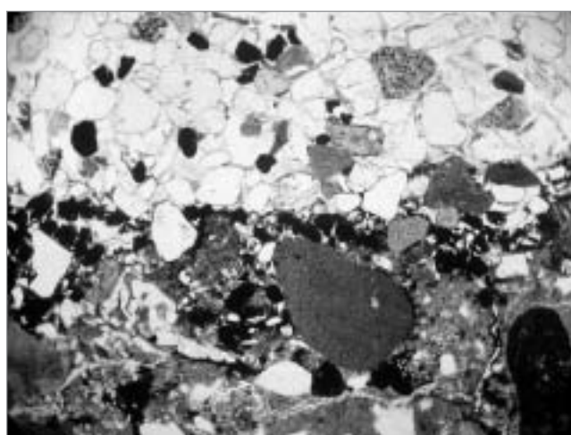
Fig. 21. Gombore I \gamma , microscopic view of sample 2149, the transition between the archaeological layer and the overlying sands, natural light. Cliché J.-P. Raynal
