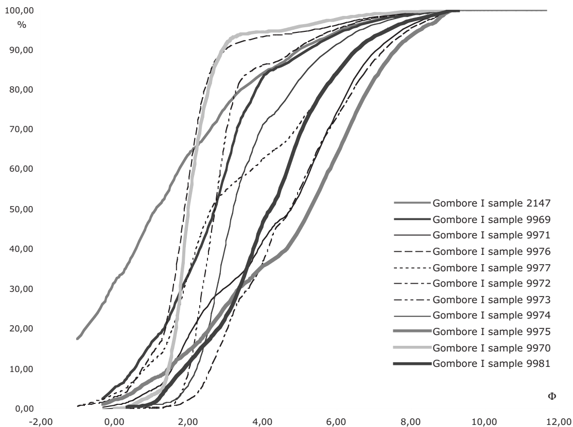
Fig. 15. Gombore I series, grain-size curves of the most representative layers.
