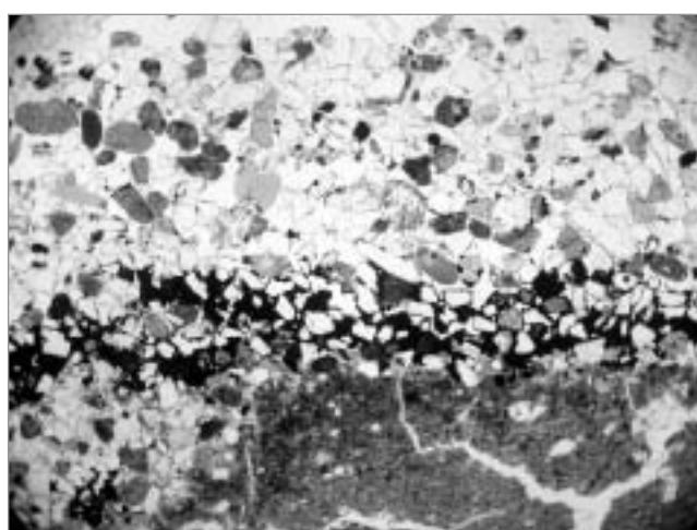
Fig. 26. Gombore II, sector 5, microscopic view of sample 2108 top, reworked tephric sands with concentration of opaques at the bottom, above silts with dessication cracks.
