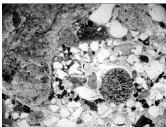
Fig. 8. Garba IV, sample 2054, thin section in bed 3.1, microscopic view in natural light, bone fragments in heterometric coarse sandy matrix. Cliché J.-P. Raynal
