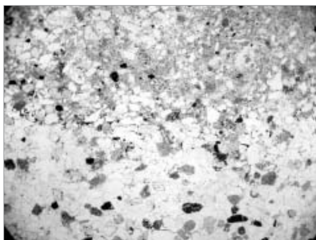
Fig. 27. Gombore II, sector 5, microscopic view of sample 2103 bottom, silts over sands, natural light.
