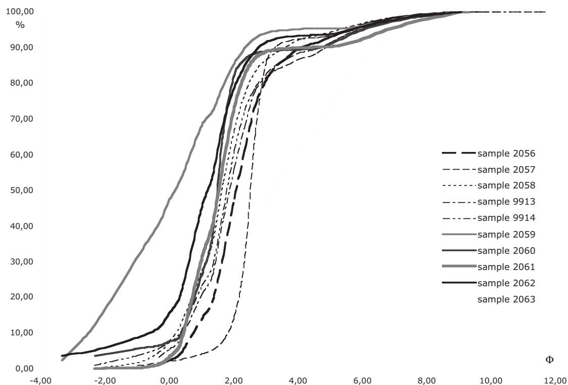
Fig. 10. Garba IV, grain-size curves of beds above archaeological Layer D.
