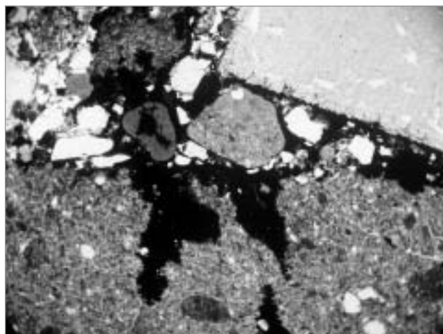
Fig. 19. Gombore I \gamma , microscopic view of sample 2149, silty sands with desiccation cracks overlain by the archaeological layer, natural light. Cliché J.-P. Raynal
