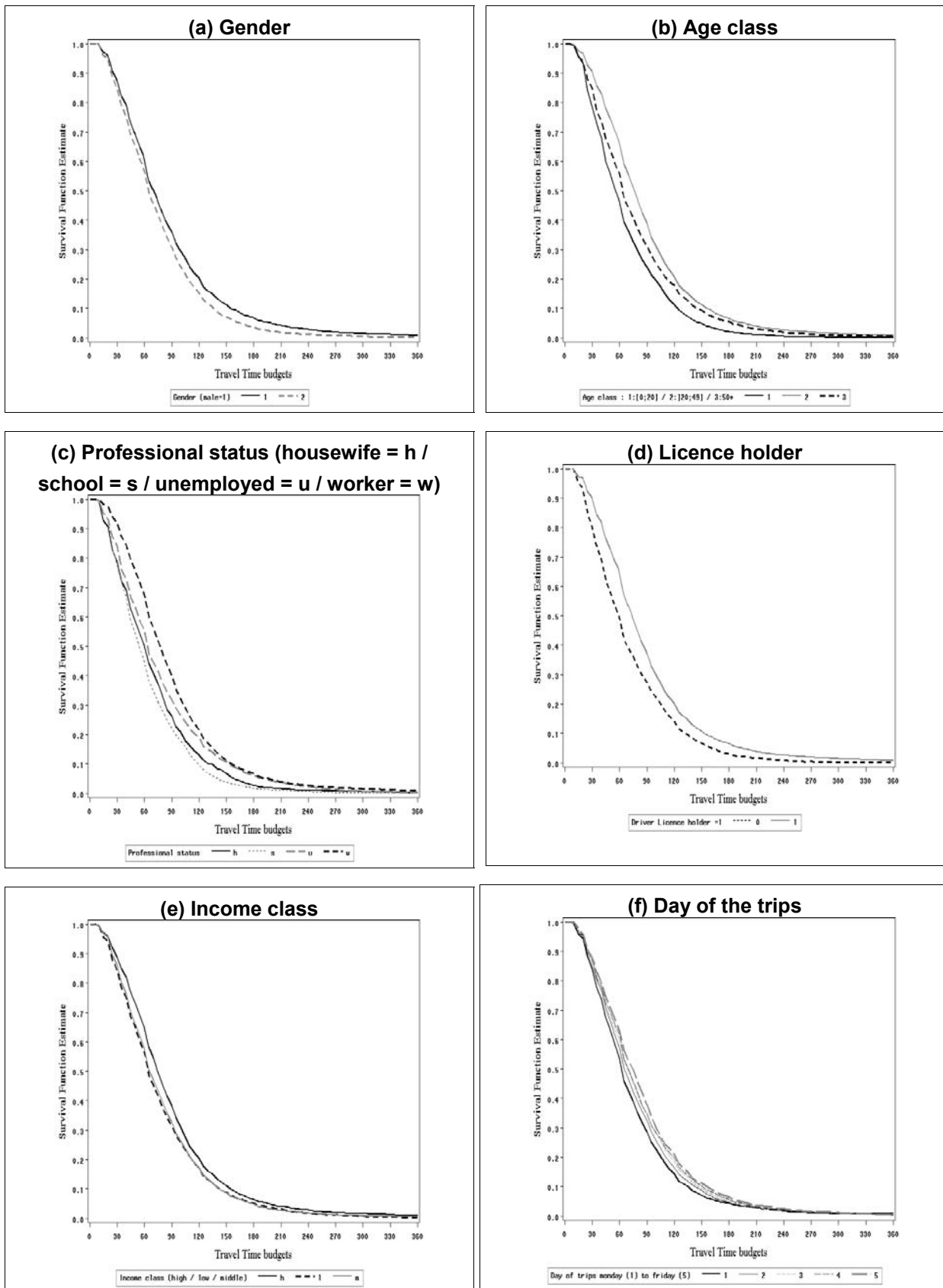
Figure 3 Survival curves
