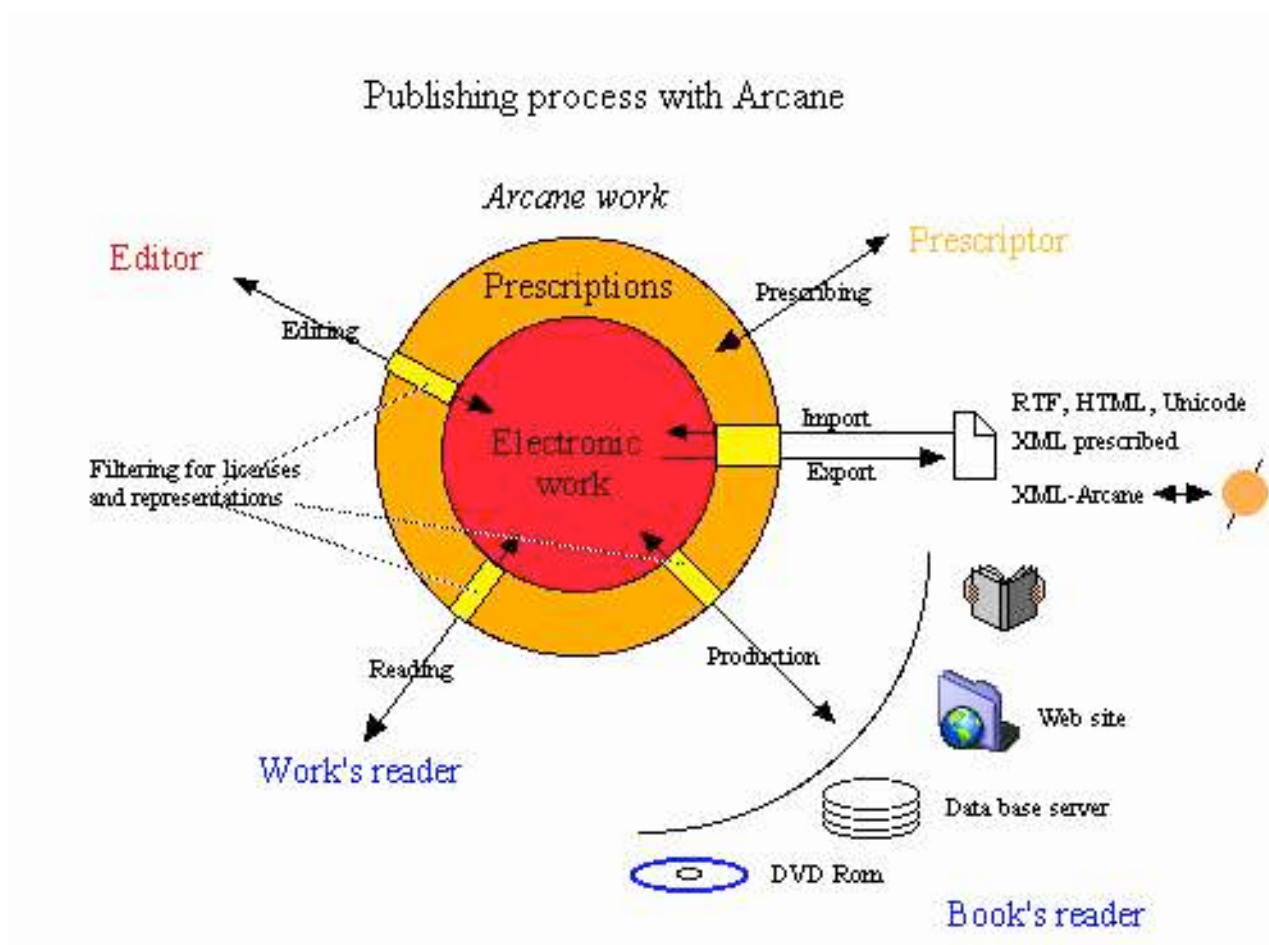
Figure 7 - Publishing process
