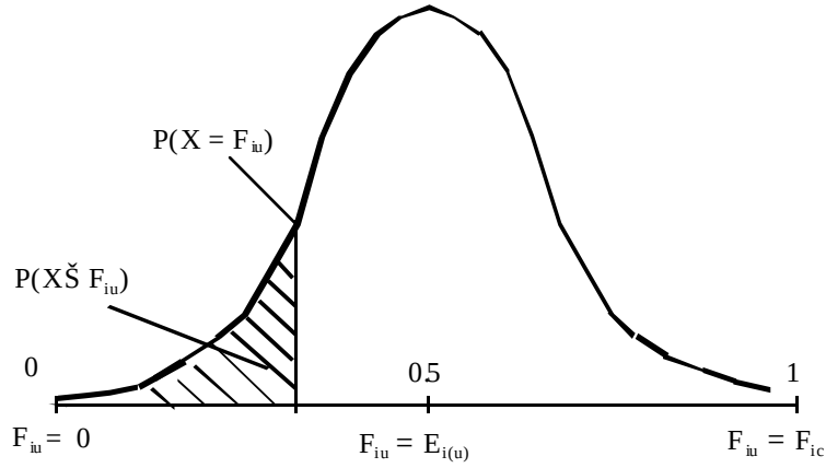
Fig. 1. Theoretical distribution of the results of Formula (3)
