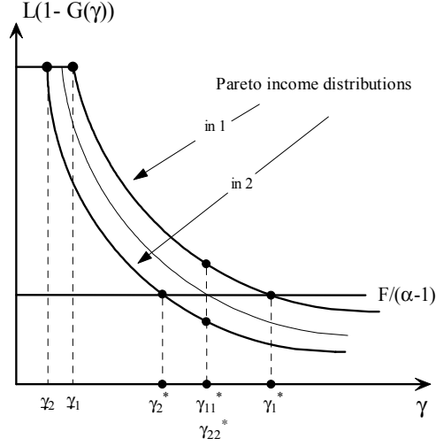
Figure 1: Pareto income distributions and share ownership in equilibrium with similar population size in both trade partners.
