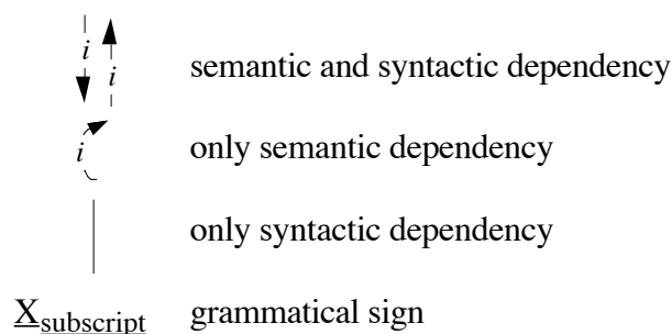
Figure 3: Graphical conventions for the derivation structure
