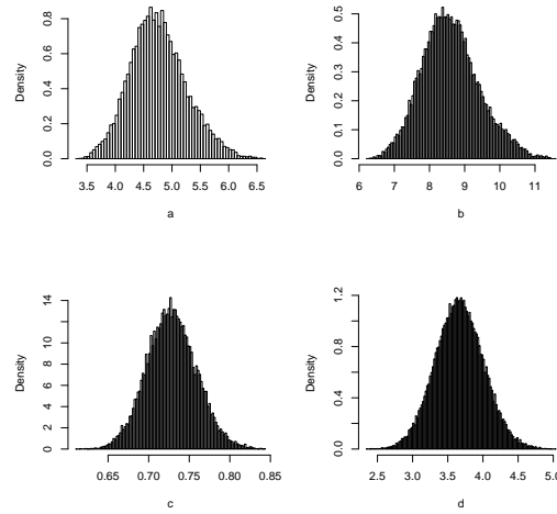
Figure 4: e = 0.01 : histograms of the last 150,000 MCMC iterations
