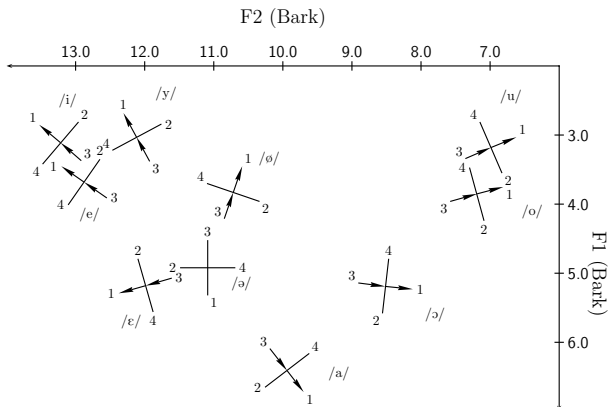
Figure 3: Order effects predicted by the neutralization hypothesis. Discrimination is easier when the stimulus presented first is located closer to [ə].
