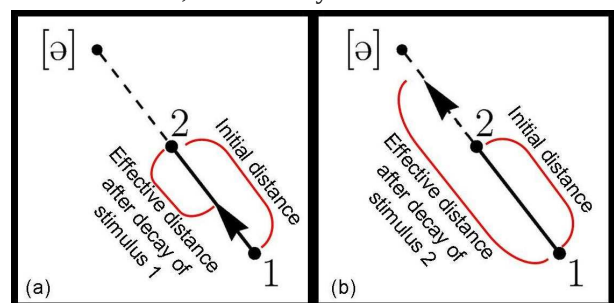
Figure 1: Direction of decay predicted by the neutralization hypothesis for stimuli 1 and 2 in the order 1-2 (a) and in the order 2-1 (b). In (a), 1 moves toward [ə] and, at the same time, toward stimulus 2; in (b), stimulus 2 moves toward [ə] but this time, further away from 1.
