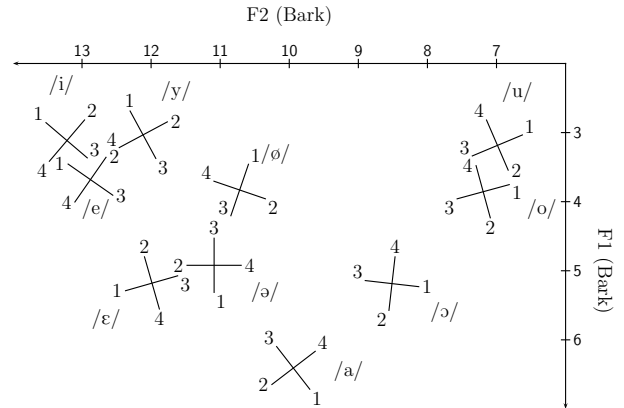
Figure 2: F1-F2 plot of the fifty synthesized stimuli. In the center of each cross lies the prototype. Neighbors (N) 1 and 3 lie on the axis pointing toward [ə].
