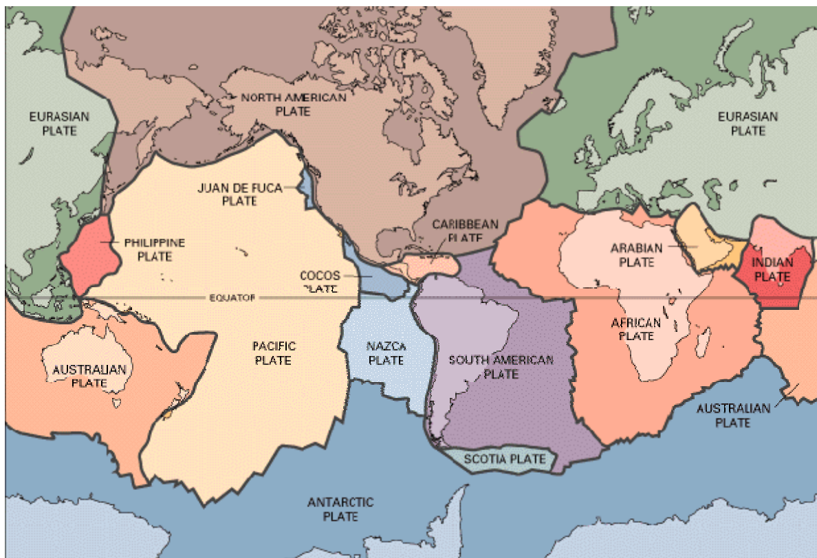
Figure 4 : Tectonic plates
