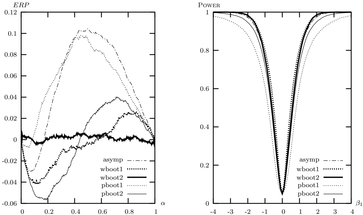
Figure 2: ERP and POWER of t -test, wild vs. pairs bootstrap: base case
