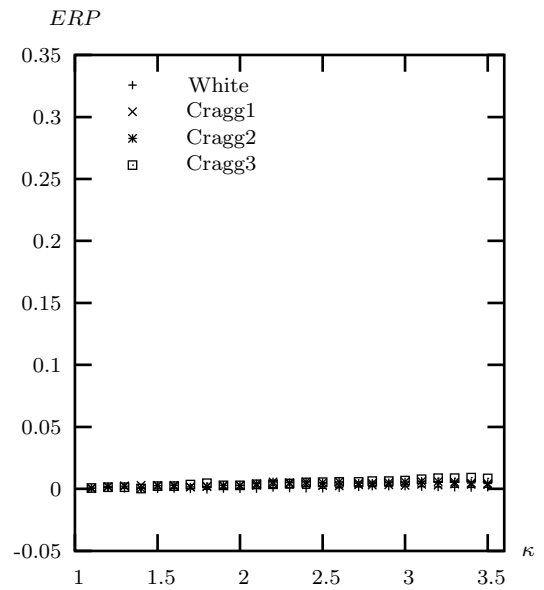
Fig 4: Bootstrap-restricted residuals
