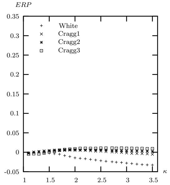
Fig 2: Aymptotic-restricted residuals
