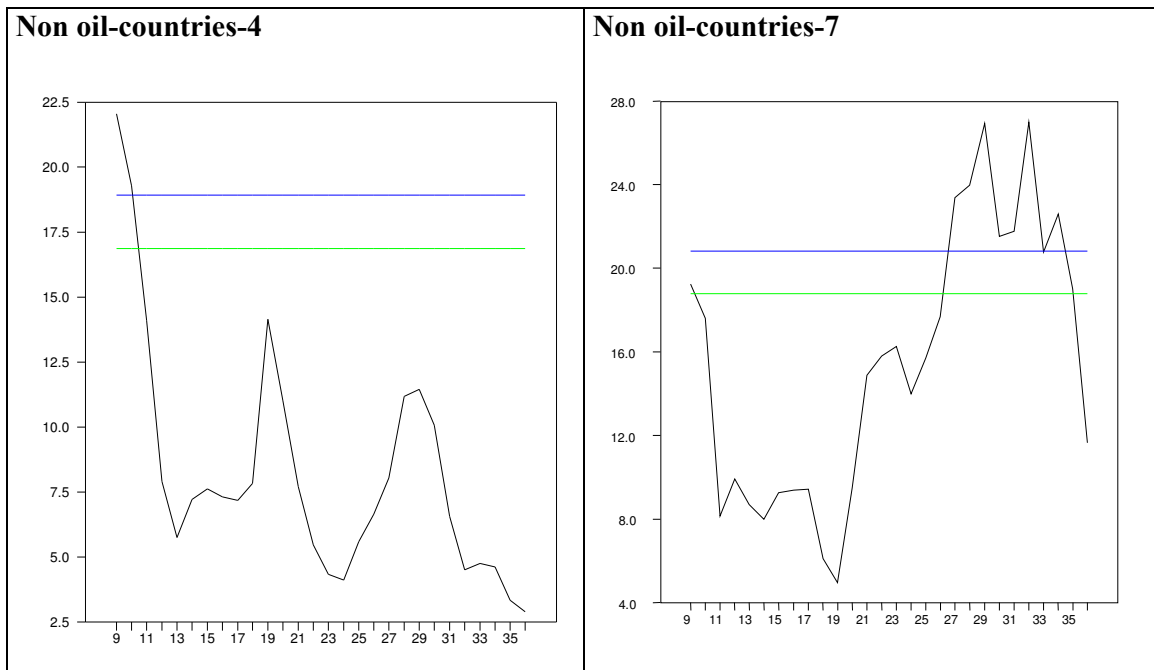
The lines correspond to the critical values tabulated by Andrews (1993b) at the 5 and 10 % level.
