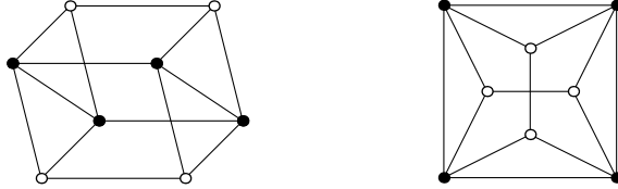
Figure 1: The two smallest double split graphs: the double-diamond and L(K_{3,3} \setminus e)
