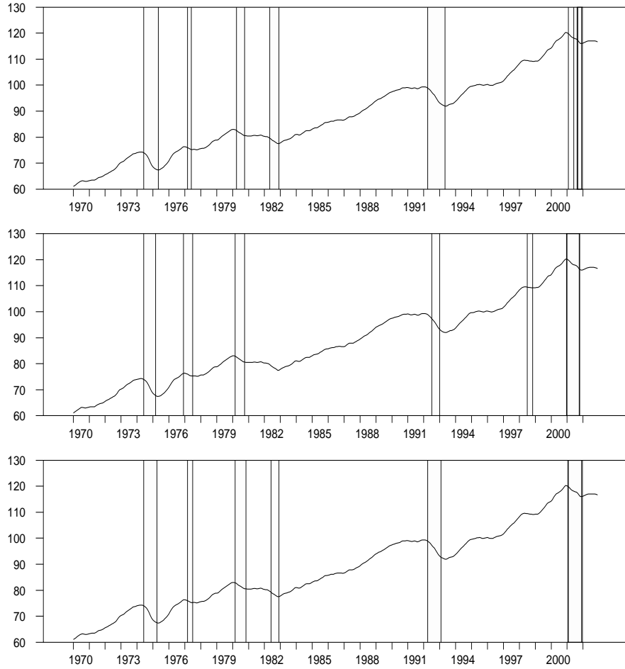
Figure 3: Industrial recession dates estimated by the 2-regime SETAR with lagged variable as transition variable (top graph), by the 2-regime SETAR with differenced lagged variable as transition variable (middle graph) and by the 4-regime SETAR (bottom graph).
