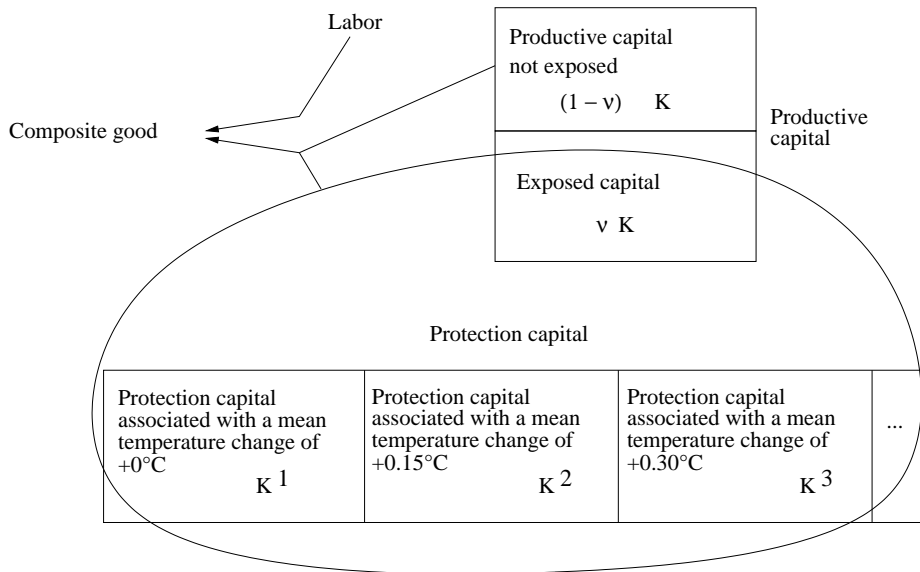
Figure 1: Three kinds of capital stock involved in adaptation to climate change. Exposed capital is the fraction of economically productive capital that is potentially impacted by climate change. Protection capital is the accumulation of specific, long-lived, non-productive resources allocated to adaptation.
