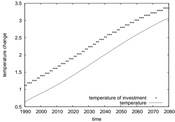
Figure 4: Optimal investment in protection capital (++) line) anticipates the atmospheric temperature (dashed line) by about two decades, or half a degree.
