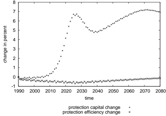
Figure 5: The balance of costs. Compared to the BAU, the optimal trajectory invests more in protection capital, but the efficiency losses stay small.
