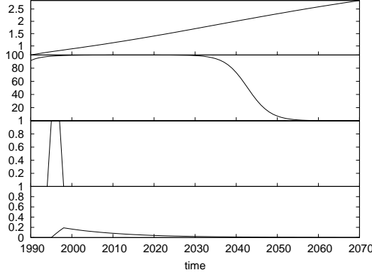
Figure 3: Evolution of the type 10 protection capital, associated with a temperature increase of 1.26°C. From top to bottom: global temperature increase \theta_t , efficiency of the capital g(\theta_t - \theta^{10}) , investment in that type of capital scaled by the total amount of investment in protection capital \frac{i_t^{10}}{\sum_j i_t^j} and capital 10 stock scaled by the total amount of protection capital.
