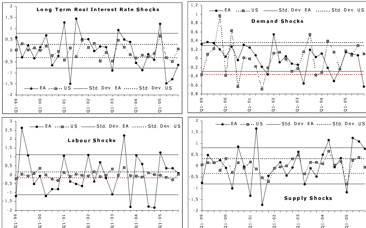
Figure 8: Historical shocks
