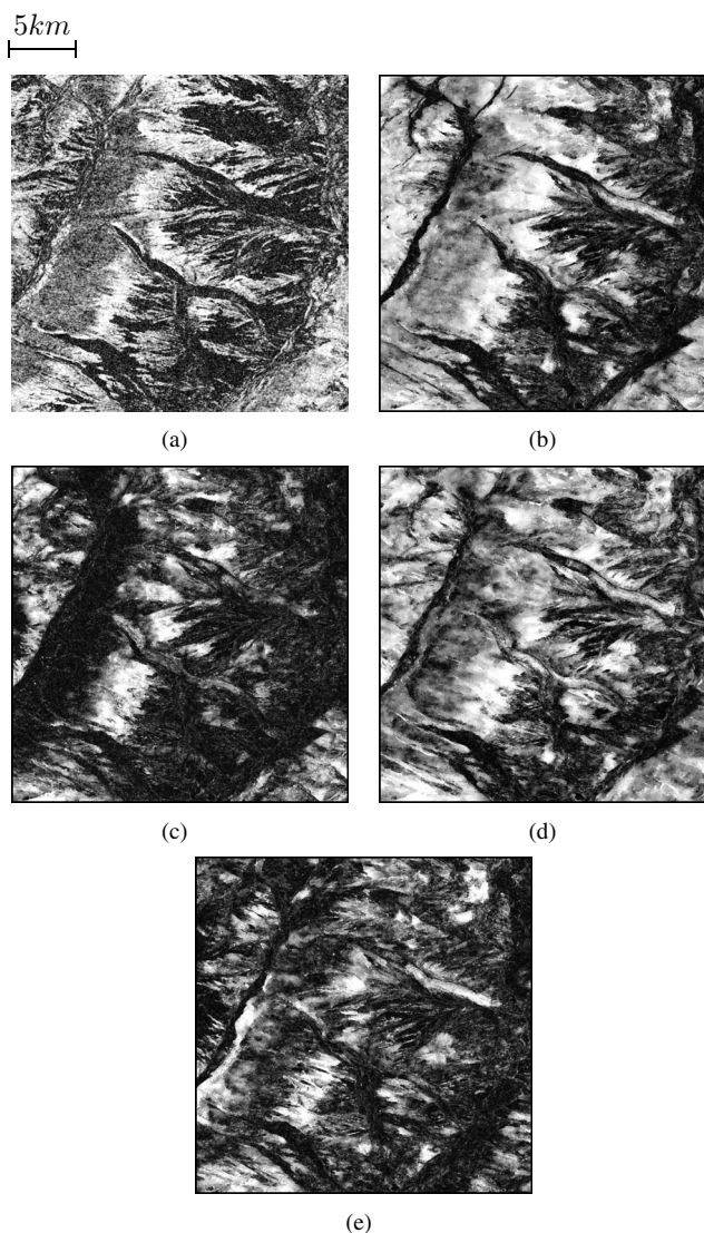
Fig. 1. ERS-1/2 tandem interferograms over the Mer de Glace - Leschaux and Argentière glaciers area ( 1024 \times 1024 pixels). Coherence filtered by amplitude driven adaptive neighborhood. (a) 9/10 Jul.95, (b) 22/23 Oct.95, (c) 31 Dec.95/1 Jan.96, (d) 10/11 Mar.96, (e) 14/15 Apr.96
