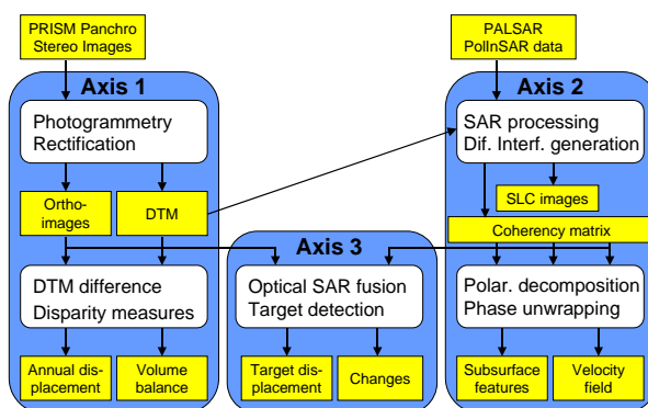
Figure 6. Research axes on PRISM and PALSAR data to monitor temperate glacier activity
