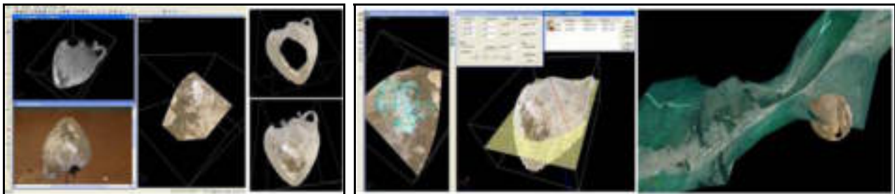
Fig. 6. On the left: Synoptic view of method combination; on the left laser range and programmatic photo, the mesh derived from photogrammetry in the central icon, and on the right the artificial hole in the laser- derived mesh close through the mesh derived from photogrammetry
