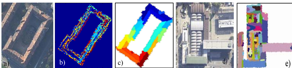
Figure 5. Roof planes detection results
