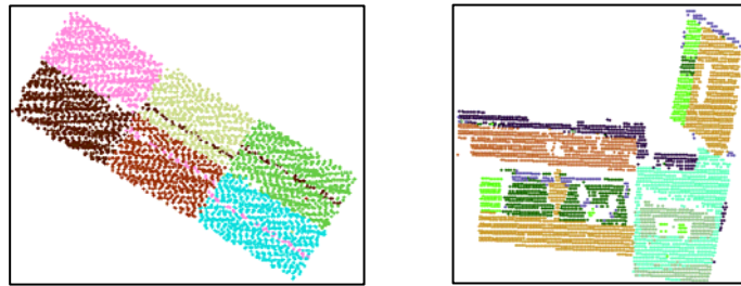
Figure 1. Roof plane detection result using the RANSAC. The colours represent the different building roof planes a) Point density: 7 pts/m 2 . b) Point density: 1.3 pts/m 2 .
