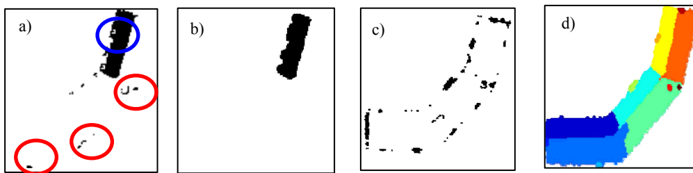
Figure 2. a) DSMb of the detected plane (yellow plane in Fig.2d); b) DSMb of the improved detected plane; b) DSMb of the remaining points after detecting the roof planes; d) Final result of roof planes detection.
