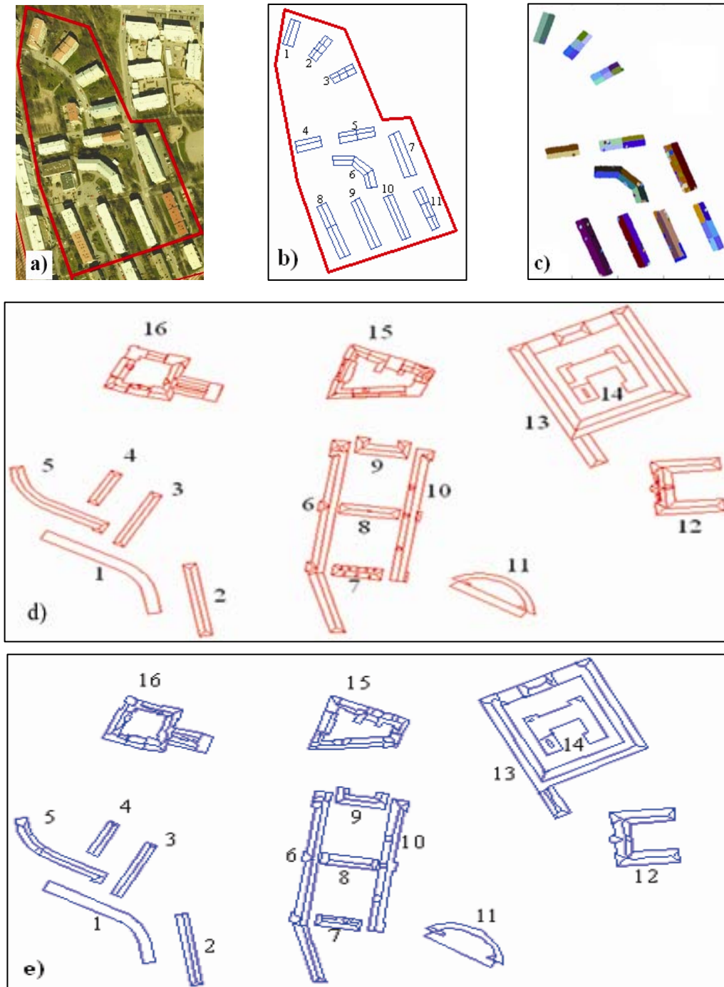
Figure 6. Estimation of the accuracy of the automatic plane detection using the extended RANSAC algorithm
