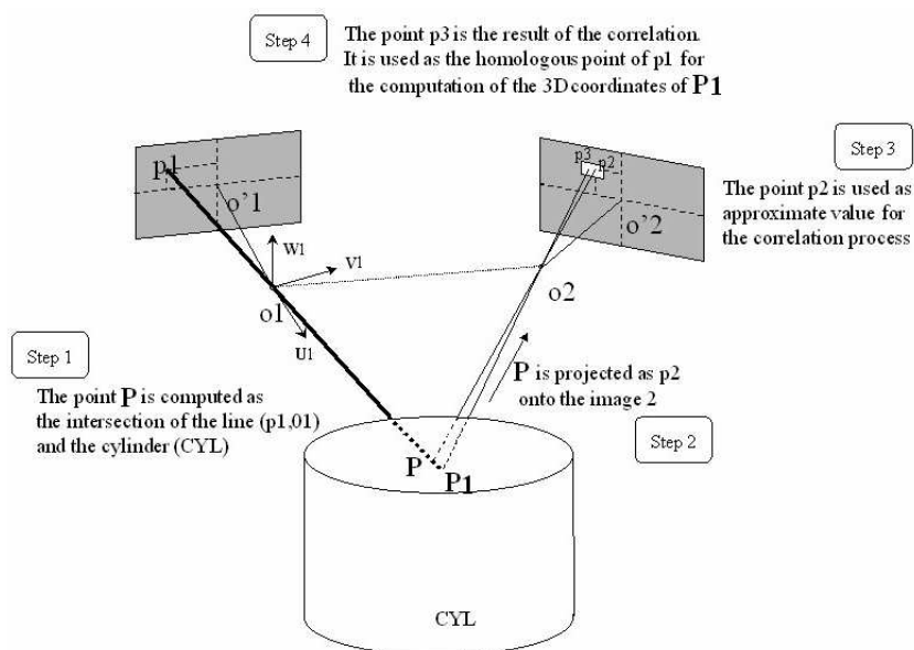
Figure 1. Steps of the I-MAGE process in ARPEUTEUR.
