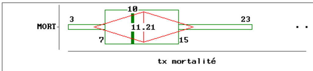
Box Plot
