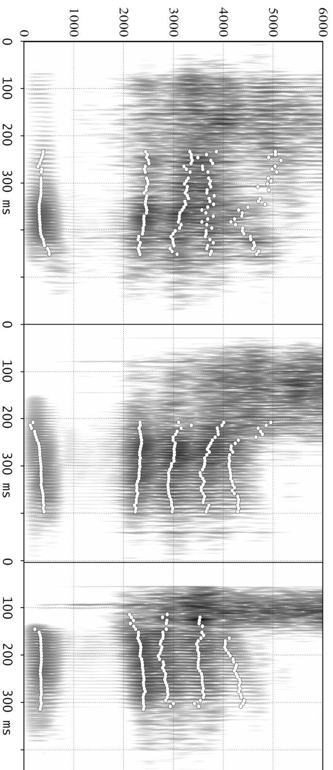
Spectrogram 1b: /i/, realised as [ji] Spectrogram 2b: /ɛi/ Spectrograms 1b, 2b and 3b are based on data from an adult male subject. The superimposed dots indicate the frequency of formants F1 to F5 as evaluated by the software PRAAT.
