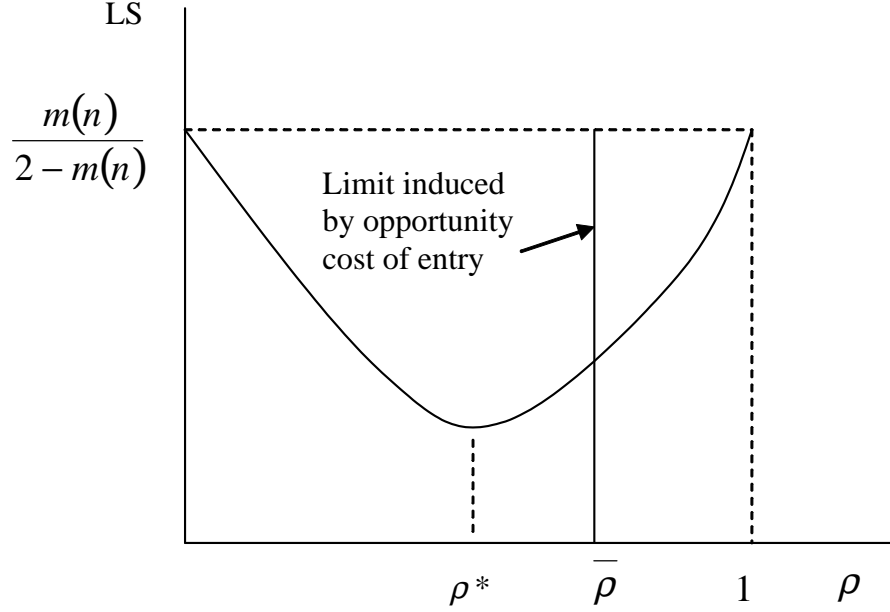
Figure 1: Labor share and proportion of jobs in foreign firms. LS goes from 0 to 1 as c_F goes from infinity to c_R . The proportion \bar{\rho} corresponds to c_O = 0 .
