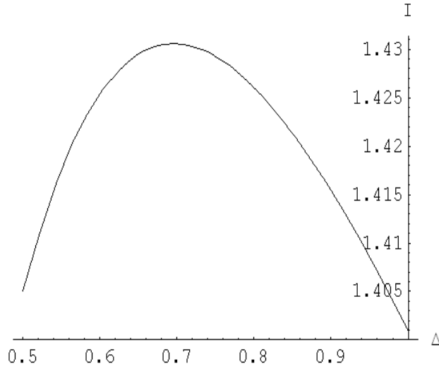
Figure 7. The effect of competition ( \Delta ) on aggregate flow of innovation (I) using n_{1a}
