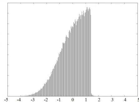
(C.b) \Delta\left(0, 1, -\frac{\sqrt{2}}{2}, 0\right)
