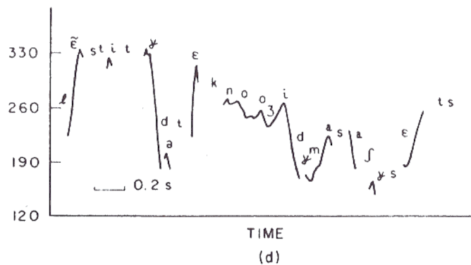
Fig. XVI-26. F_0 contours for the same phrase (l'institut de technologie du Massachusetts ...) spoken by four talkers, illustrating different strategies for grouping the words.
