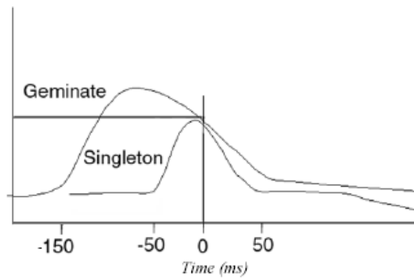
Figure 5. Illustration of the glottal opening during the production of the stops in [ittili] and [itili]. The vertical bar indicates the onset of oral release (adapted from Ridouane 2003).
