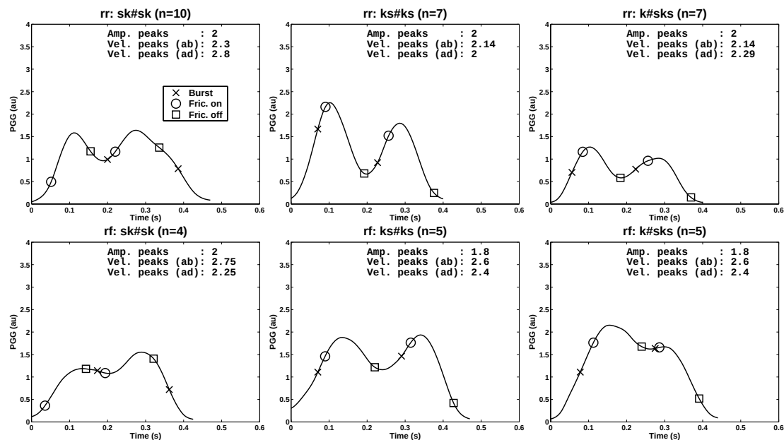
Figure XXX, 8. Averaged glottal abduction pattern for /sk#sk/, /ks#ks/ and /k#sks/. Symbols as in Fig. 2.
