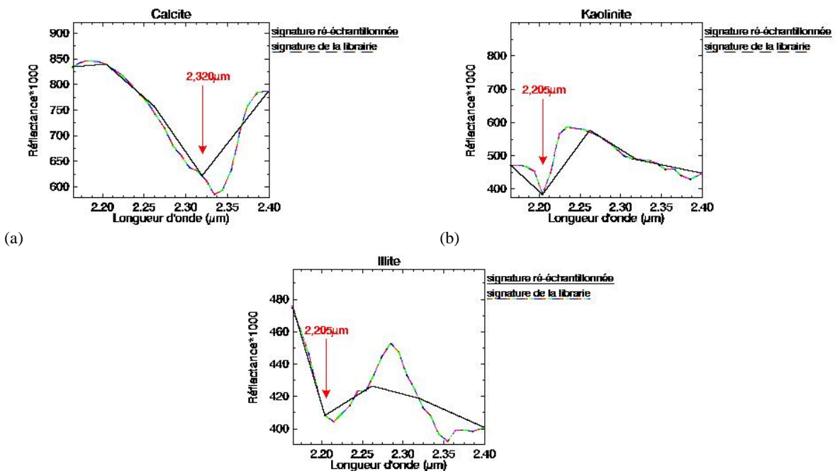
Figure 5 : Spectre de réflectance original de la librairie USGS et ré-échantillonné de la calcite (a), la kaolinite (b) et l'illite (c). Figure 5: USGS Original and resampled reflectance spectra of: calcite (a), kaolinite (b) and illite (c).
