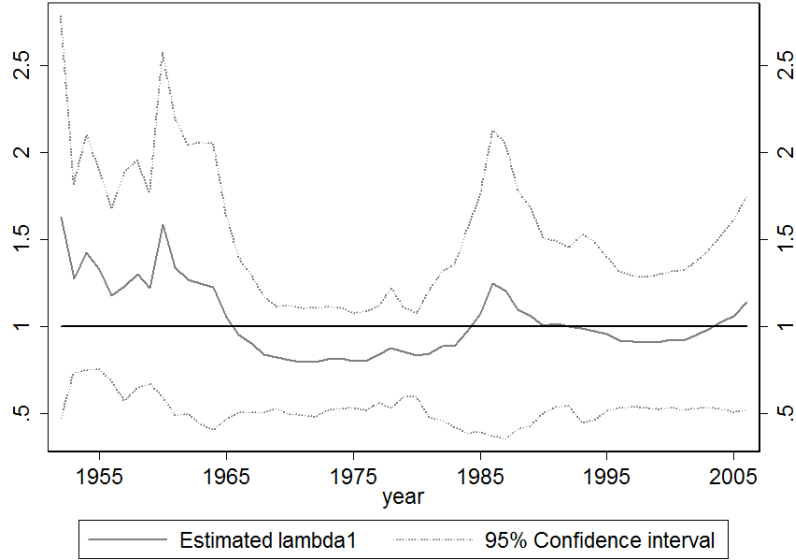
Figure 7: Estimated \lambda_1
