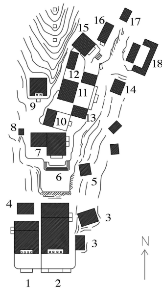
III. 6. The layout of the Badγar coyiling süme [4] (Urad, Ulaγancab league), central part, before 1947. Nagao Gajin, 1991 [1947], fig. 2, p. 137
