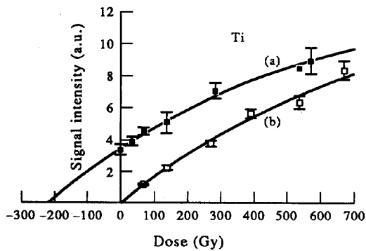
Fig. 6. DRC of the Al and Ti paramagnetic centres for sample C213; explanations: as for Fig. 3.
